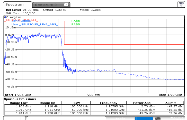
n2_5MHz_15kHz_1907.5MHz_DFT-s-OFDM QPSK_RB25@0
