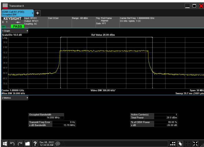
n2_15MHz_15kHz_1880MHz_DFT-s-OFDM 256 QAM_RB75@0
