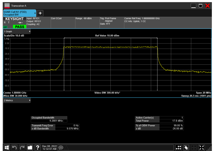
n2_10MHz_15kHz_1880MHz_CP-OFDM 256 QAM_RB52@0
