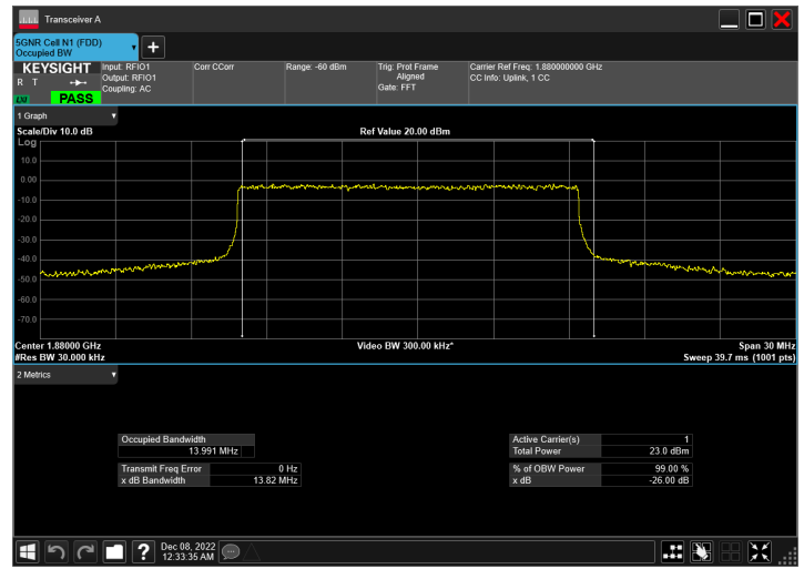
n2_15MHz_15kHz_1880MHz_DFT-s-OFDM 64 QAM_RB75@0
