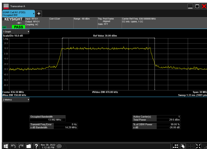
DC_2A_n5A_10MHz|15MHz_15kHz_1880MHz|836.5MHz_QP SK|CP-OFDM 64 QAM_RB1@50|RB79@0
