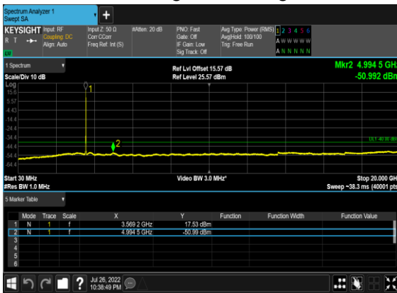
N48(20M)_DFT-s-OFDM_BPSK_Edge_1RB_Right_Low_CH
