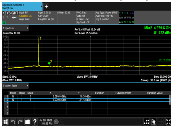
N48(20M)_DFT-s-OFDM_BPSK_Edge_1RB_Right_High_CH
