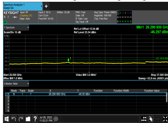
N48(20M)_DFT-s-OFDM_BPSK_Edge_1RB_Right_High_CH
