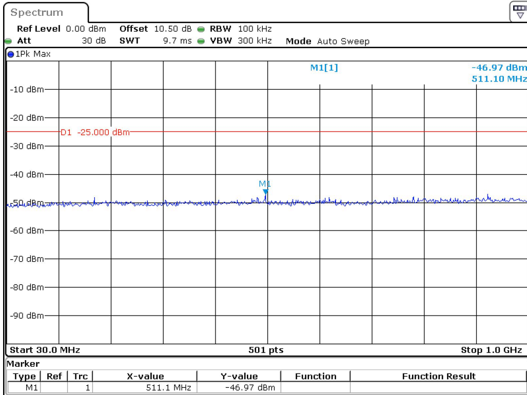
Band 7_5 MHz_Low_QPSK_RB25#0_1(30MHz-1GHz)
