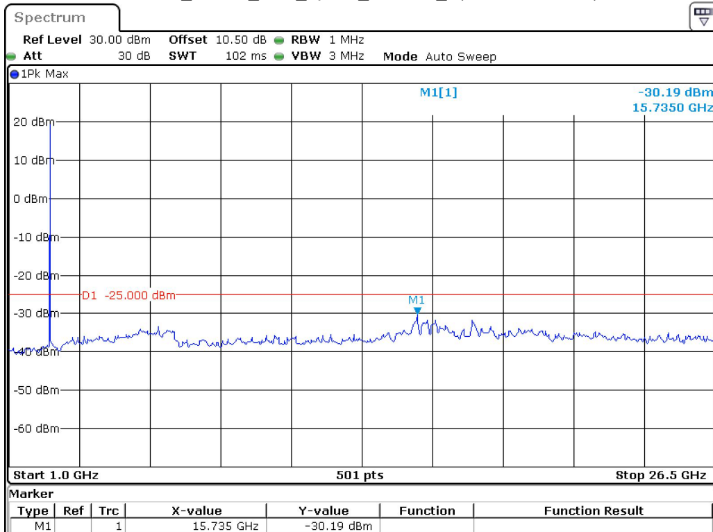
Band 7_5 MHz_Low_QPSK_RB25#0_2(1GHz-26.5GHz)
