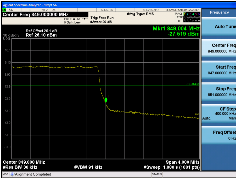
BAND 26. Upper Band Edge Plot (3M BW Ch. 27025 QPSK_RB15_Offset 0) -2
