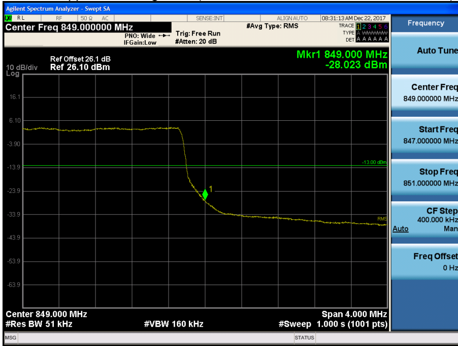
BAND 26. Upper Extended Band Edge Plot (5M BW Ch. 27015 QPSK_RB25_0) -3
