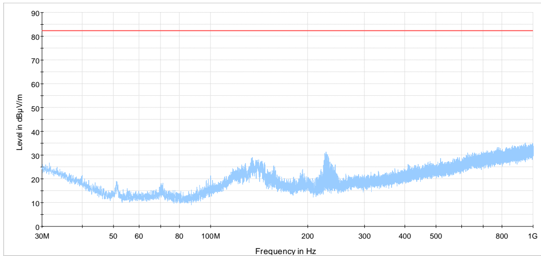
SPR 30 MHz to 1 GHz high channel — Preview Result 1-PK+ — -13dBm theoretical limit
