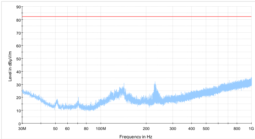
SPR 30 MHz to 1 GHz high channel — Preview Result 1-PK+ — -13dBm theoretical limit
