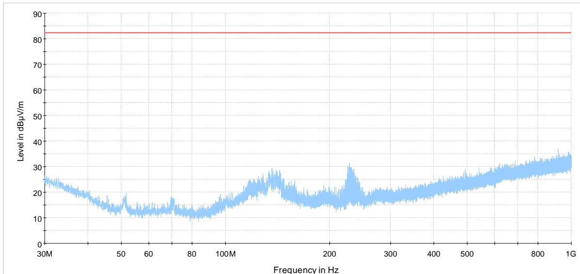
SPR 30 MHz to 1 GHz mid channel — Preview Result 1-PK+ — -13dBm theoretical limit
