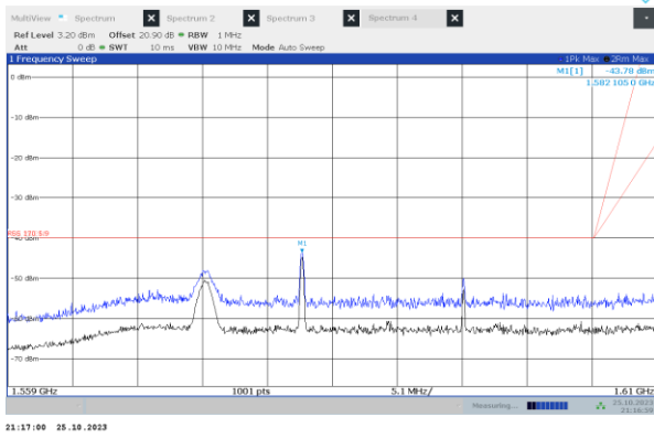
Figure 7.5-13: spurious emissions 1559–1610 MHz, Waveform Z, low channel
