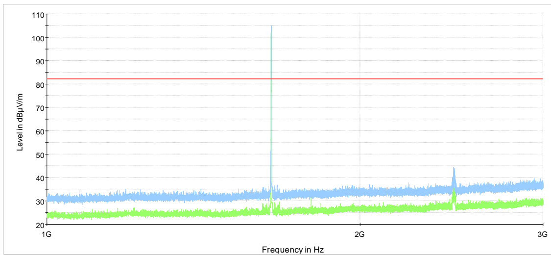
SPR 1 GHz to 3 GHz mid channel waveform — Preview Result 2-AVG — Preview Result 1-PK+ — -13dBm theoretical limit
