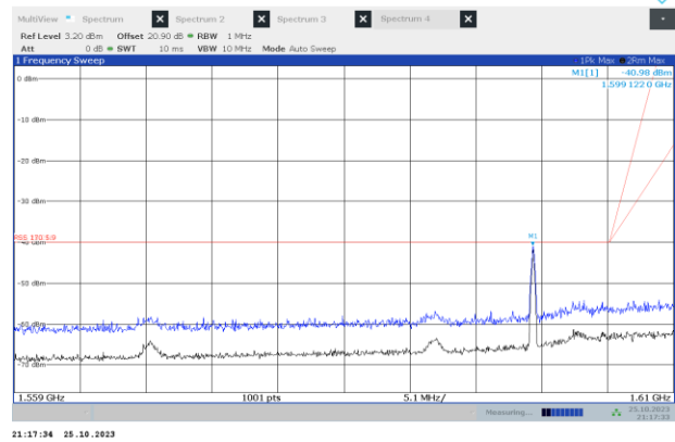
Figure 7.5-14: spurious emissions 1559–1610 MHz, Waveform Z, mid channel
