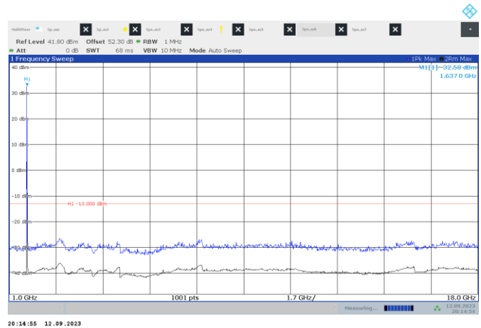
Figure 7.3-10: Conducted spurious emissions, high channel (1-18 GHz)
