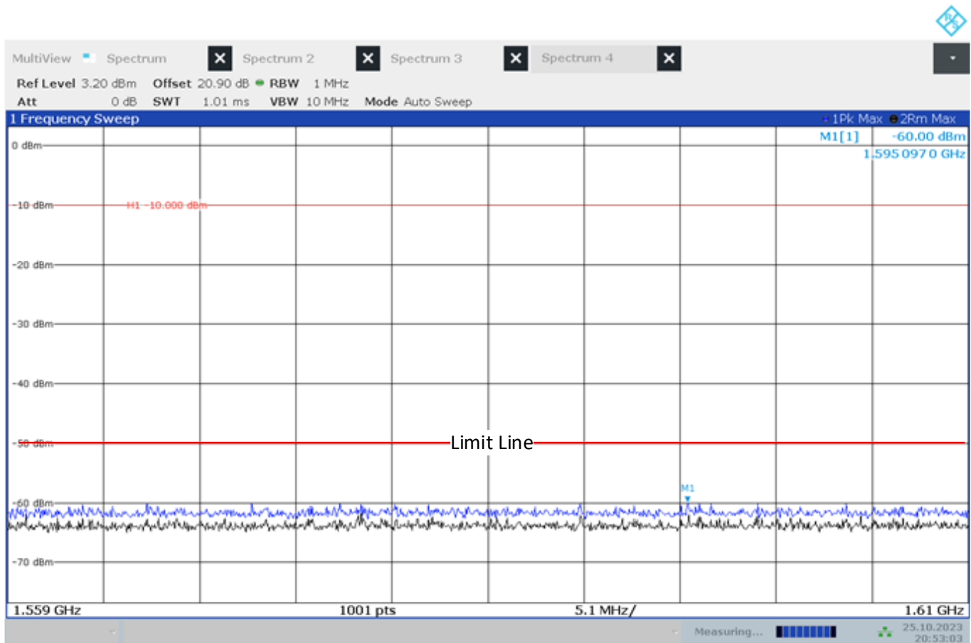
Figure 7.3-46: Radiated spurious emissions 1559–1610 MHz, carrier-off
