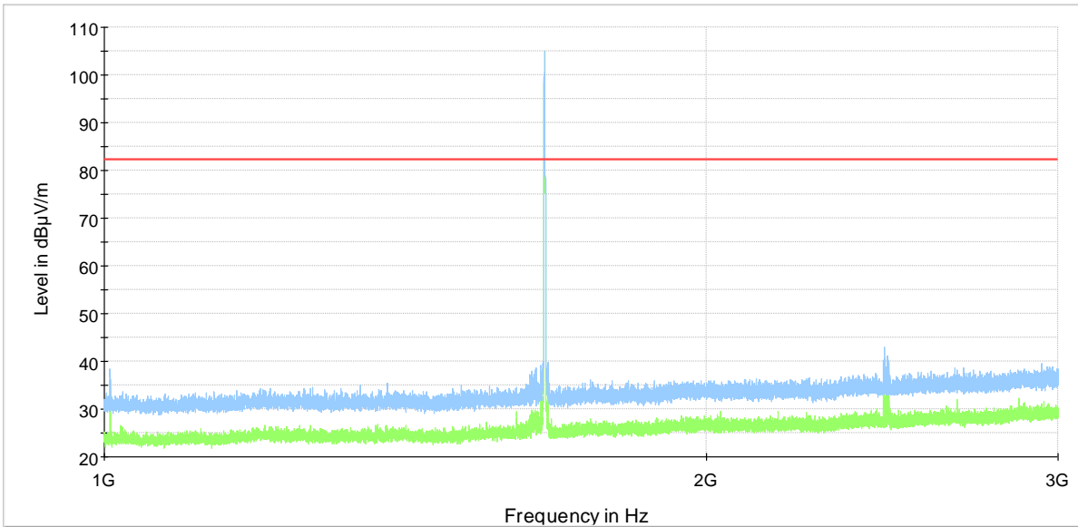
SPR 1 GHz to 3 GHz high channel — Preview Result 2-AVG — Preview Result 1-PK+ — -13dBm theoretical limit
