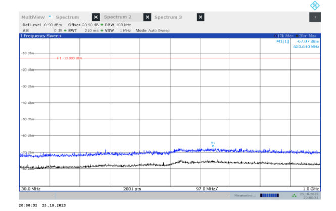
Figure 7.3-9: Conducted spurious emissions, high channel (30-1000 MHz)
