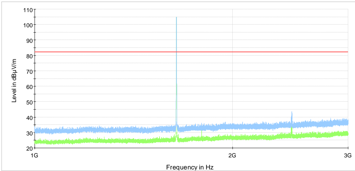
SPR 1 GHz to 3 GHz mid channel — Preview Result 2-AVG — Preview Result 1-PK+ — -13dBm theoretical limit
