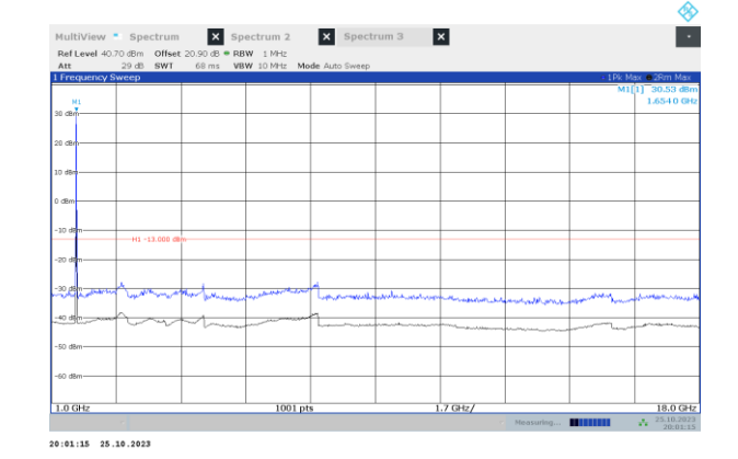
Figure 7.3-10: Conducted spurious emissions, high channel (1-18 GHz)
