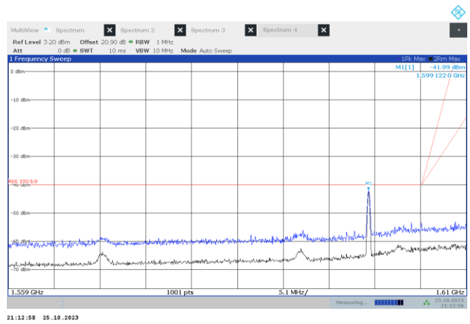
Figure 7.5-8: spurious emissions 1559–1610 MHz, Waveform T, mid channel
