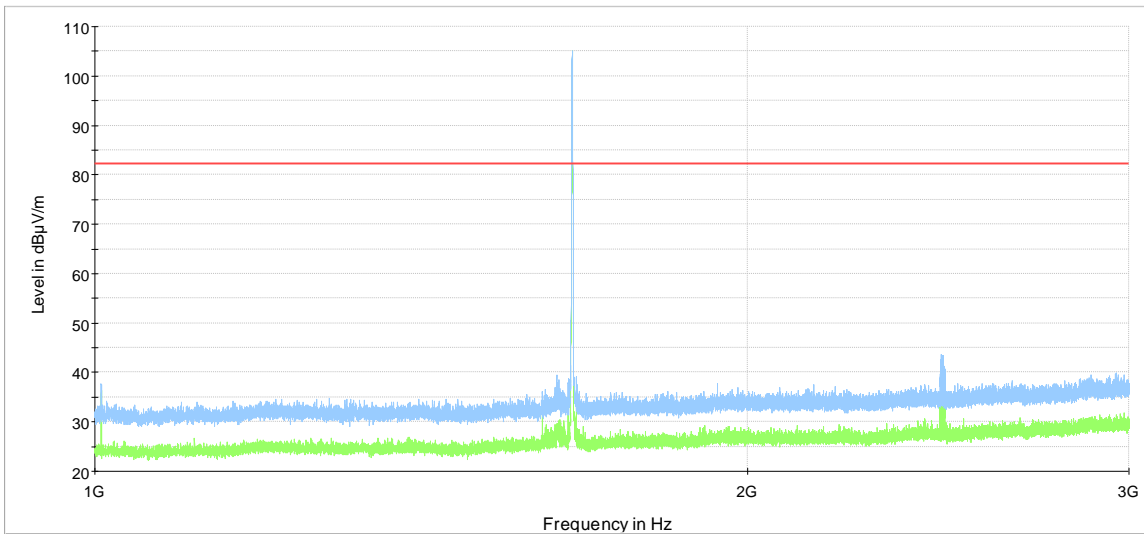
SPR 1 GHz to 3 GHz high channel — Preview Result 2-AVG — Preview Result 1-PK+ — -13dBm theoretical limit
