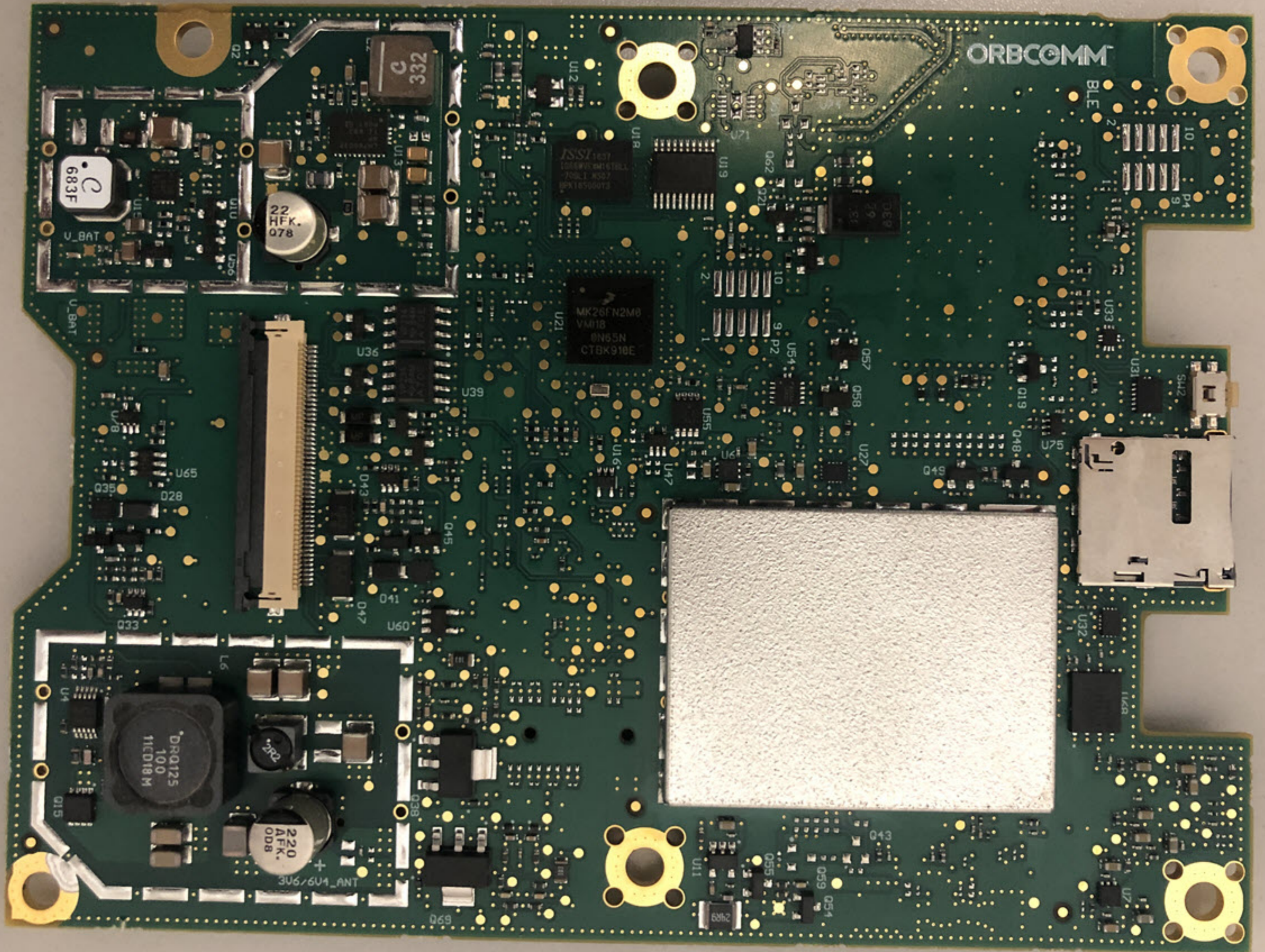
PCB top with shields
