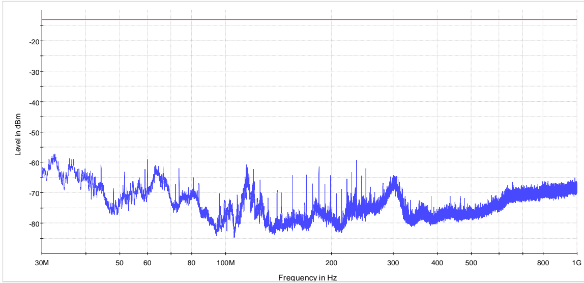
NEX-483795 RSE 30-1000 MHz Low Channel — PK+_MAXH — -13 dBm limit
