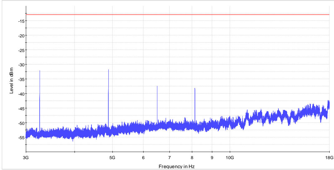
NEX-483795 RSE 3-18 GHz Low Channel — PK+_MAXH — FCC Part 25 Limit line
