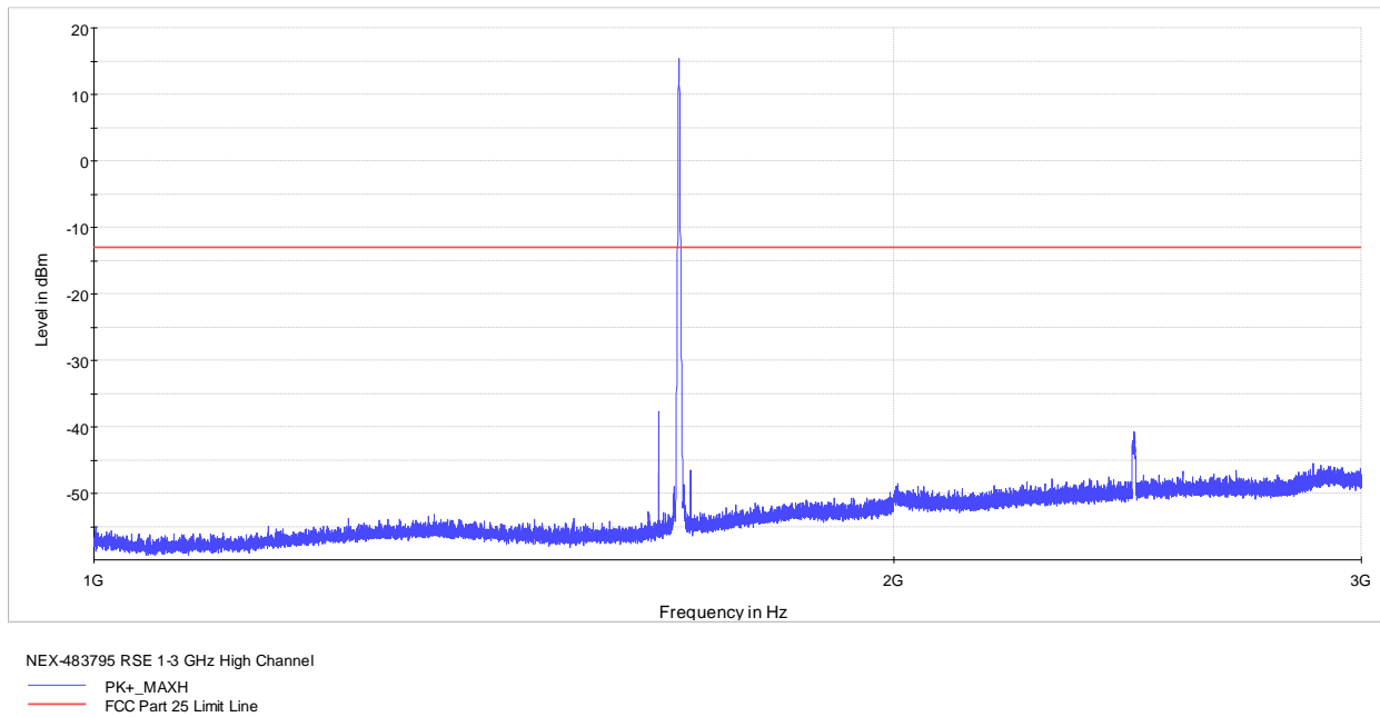
Figure 8.4-6: Radiated spurious emissions 1–3 GHz, high channel
