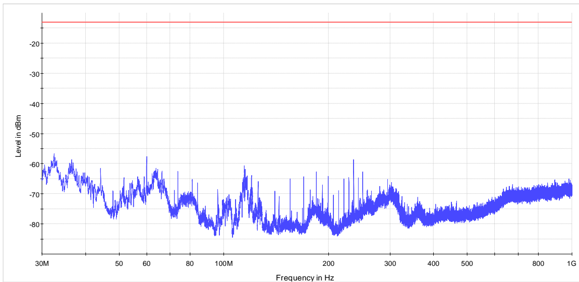
NEX-483795 RSE 30-1000 MHz High Channel — PK+_MAXH — -13 dBm limit
