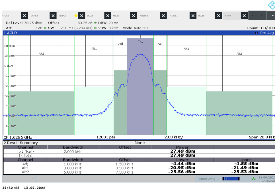
Figure 8.4-1: Conducted band edge spurious emissions outside assigned bandwidth, low channel
