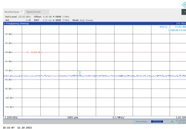
Figure 8.3-11: Conducted emissions within 1559–1610 MHz, Carrier-off state
