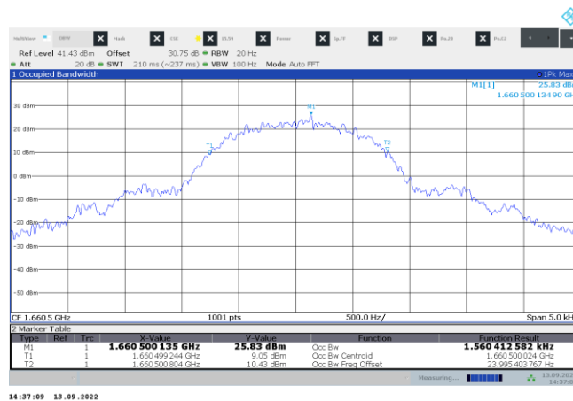
Figure 8.1-3: 99 % bandwidth on high channel
