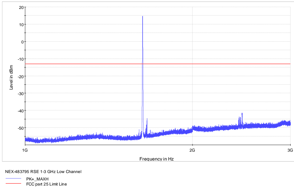
Figure 8.4-5: Radiated spurious emissions 1–3 GHz, low channel
