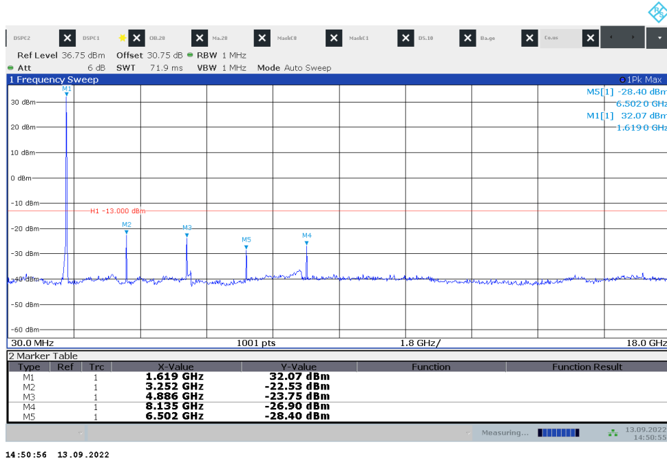
Figure 8.4-9: Conducted spurious emissions, low channel
