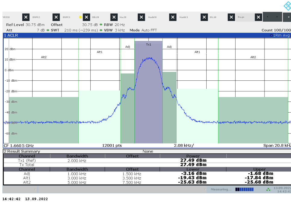
Figure 8.4-2: Conducted band edge spurious emissions outside assigned bandwidth, high channel
