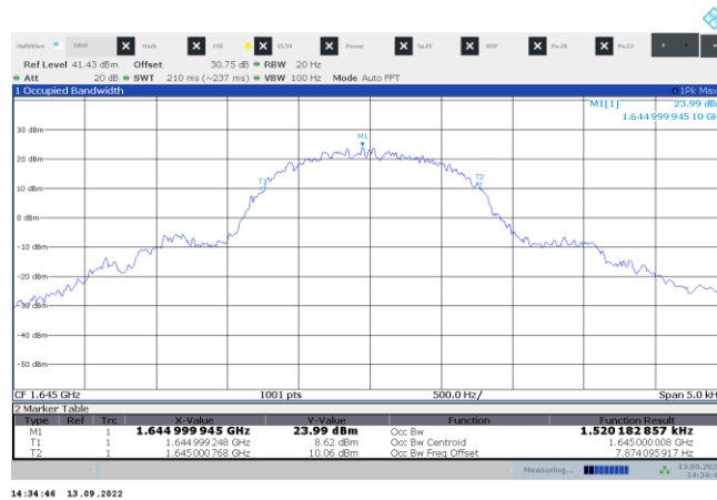
Figure 8.1-2: 99 % bandwidth on mid channel
