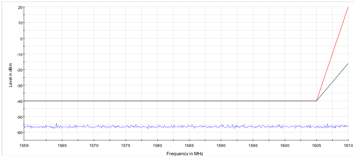
NEX-483795 RSE 1.559-1.610 GHz High Channel
