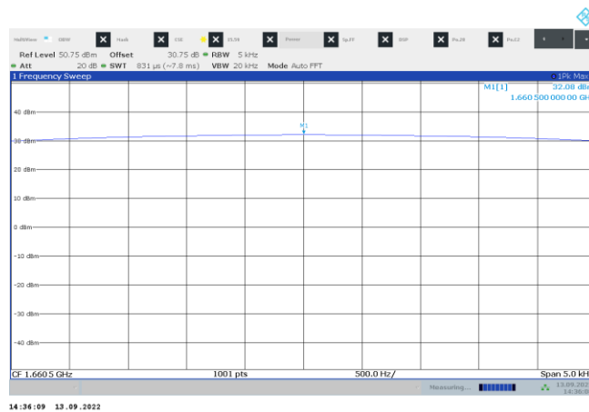
Figure 8.2-3: Conducted peak output power, high channel
