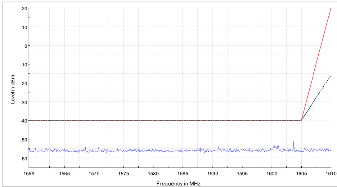
NEX-483795 RSE 1.559-1.610 GHz Low Channel
