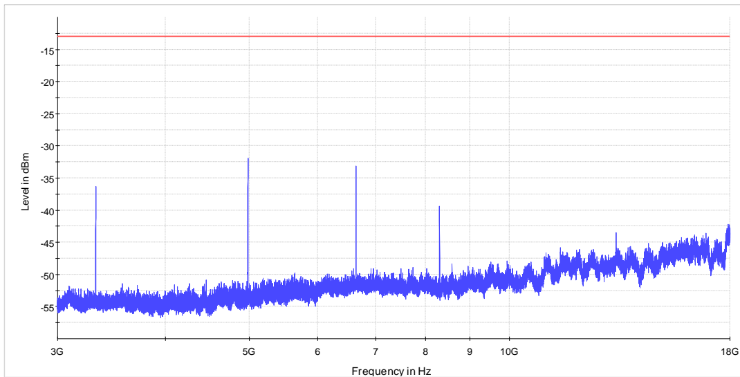
NEX-483795 RSE 3-18 GHz High Channel — PK+_MAXH — FCC Part 25 Limit line
