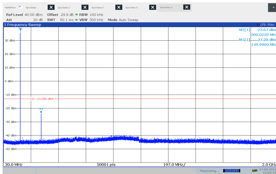
Figure 8.3-6: Conducted spurious emissions, low channel
