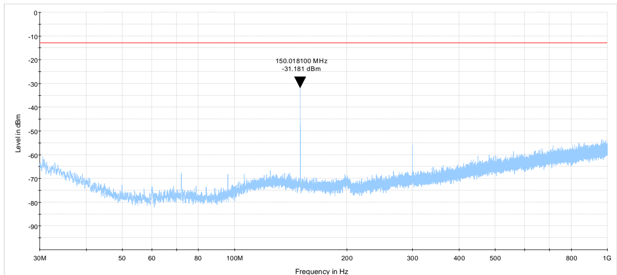
Figure 8.3-2: Spurious emissions below 1 GHz, low channel
