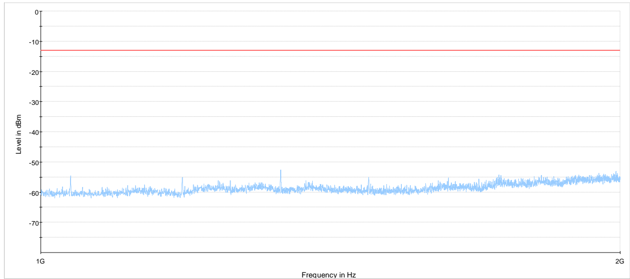
NEX-442937 Radiated spurious above 1GHz, low channel Preview Result 1-PK+ -13 dBm Limit
