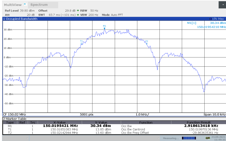
Figure 8.1-1: 99 % bandwidth on low channel
