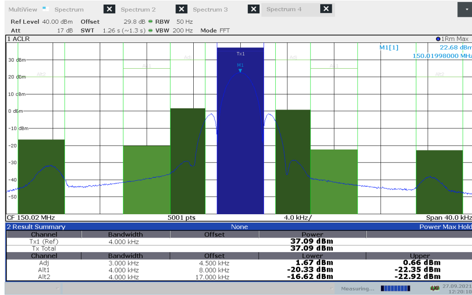
Figure 8.3-1: Out-of-band unwanted emissions, low channel
