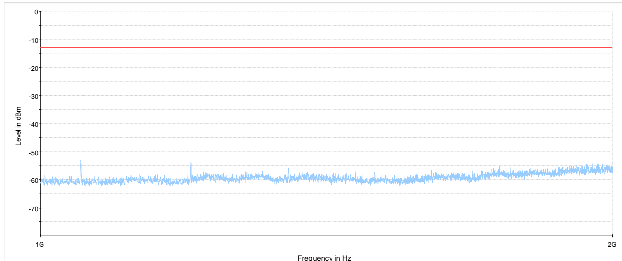
NEX-442937 Radiated spurious above 1GHz, high channel Preview Result 1-PK+ -13 dBm Limit
