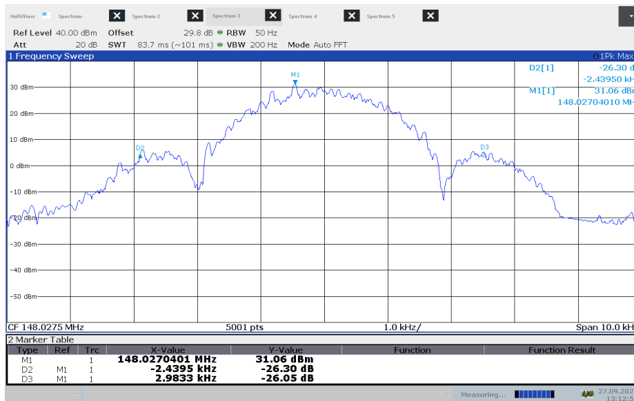
Figure 8.1-3: 26 dB bandwidth on low channel
