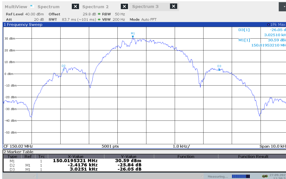
Figure 8.1-3: 26 dB bandwidth on low channel
