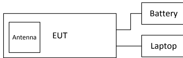
Figure 3.6-1: Setup diagram
