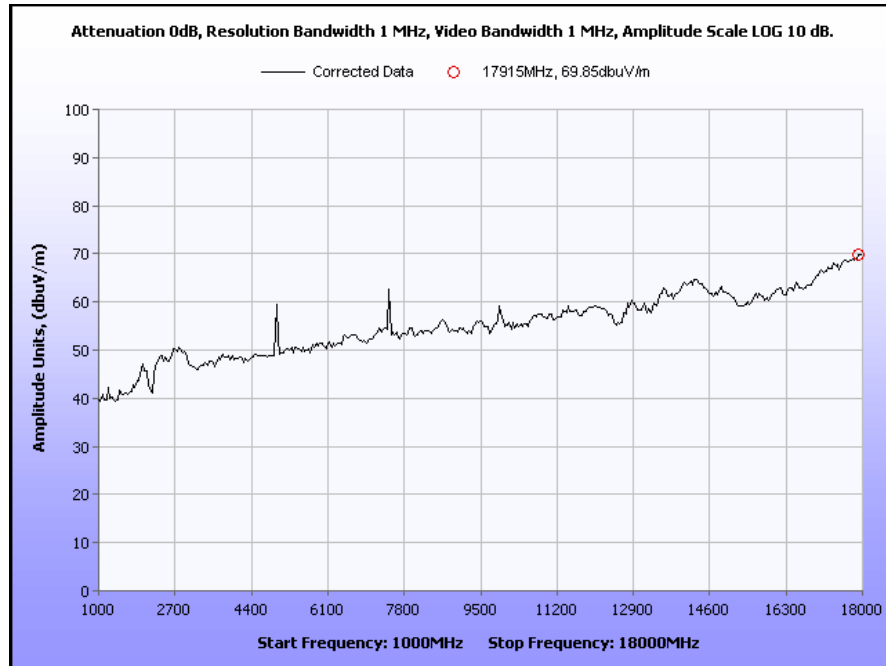
Plot 14. Radiated Harmonic Emissions, High Channel
