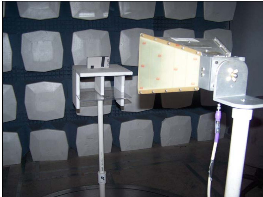
Photograph 4. Radiated Harmonic Emissions, Test Setup
