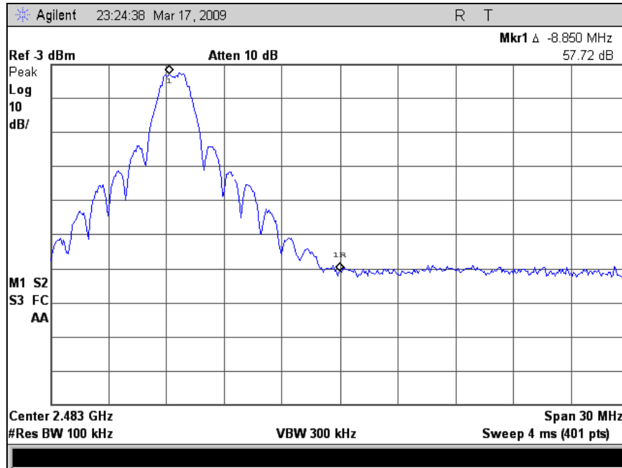
Plot 29. Spurious Conducted Emissions, Upper Band Edge
