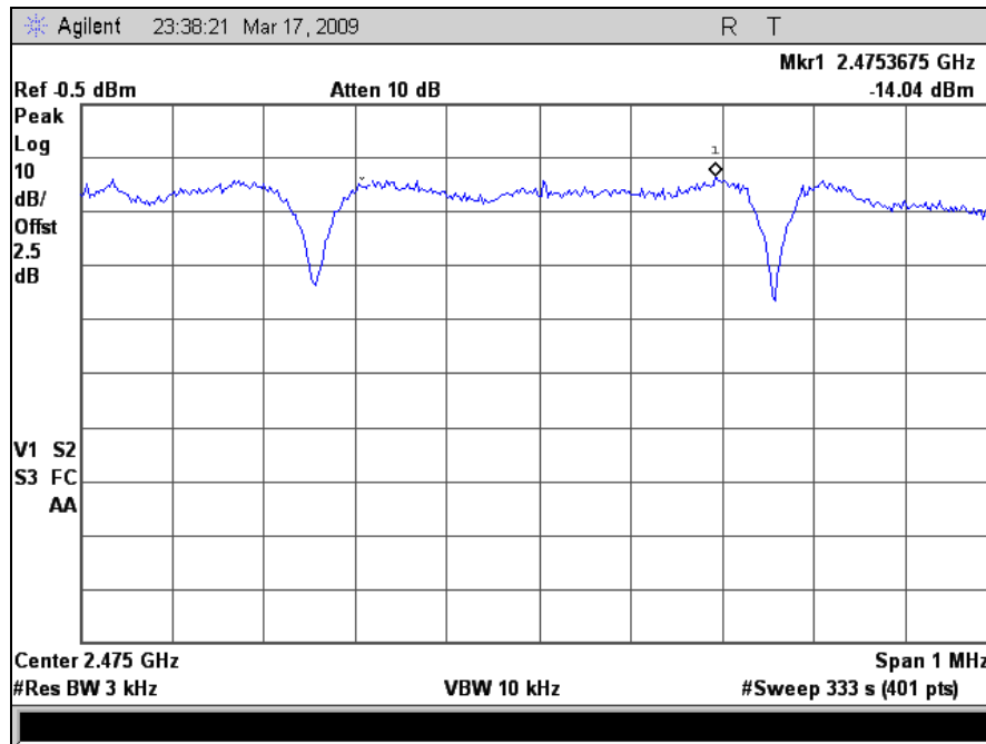
Plot 32. Peak Power Spectral Density, High Channel
