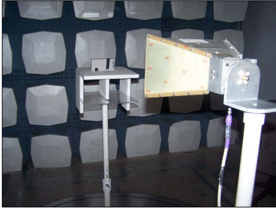
Photograph 5. Band Edge, Test Setup
