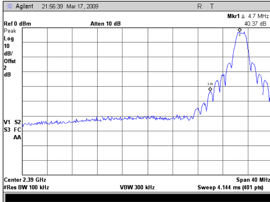
Plot 28. Spurious Conducted Emissions, Lower Band Edge
