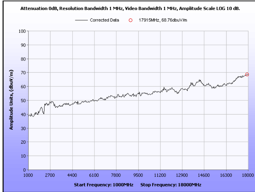
Plot 12. Radiated Harmonic Emissions, Low Channel
