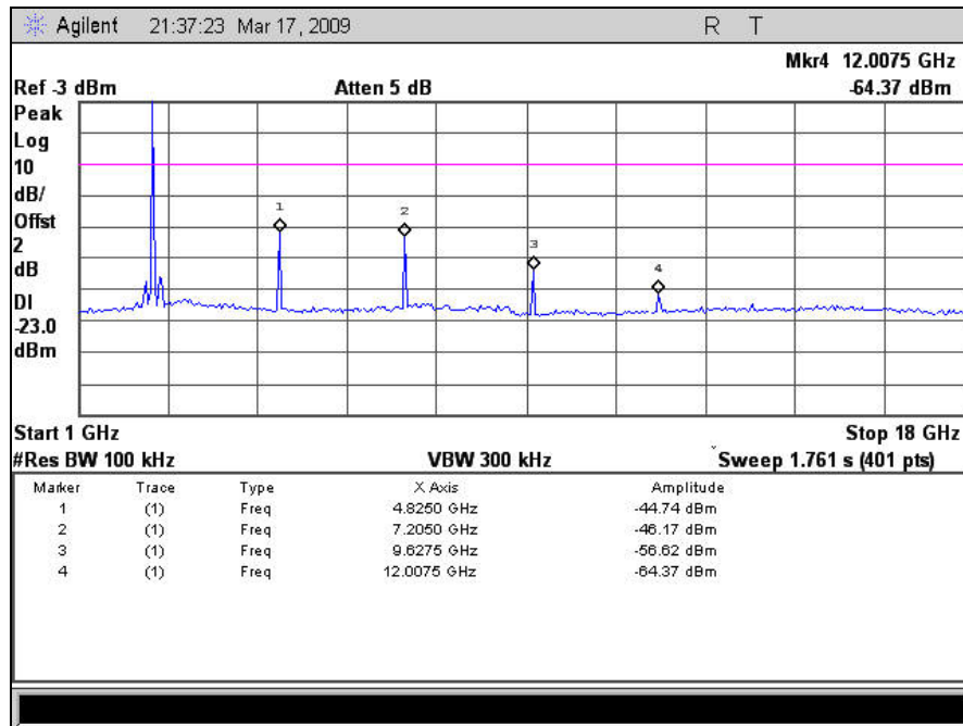
Plot 20. Spurious Conducted Emissions, Low Channel, 1 GHz – 18 GHz
