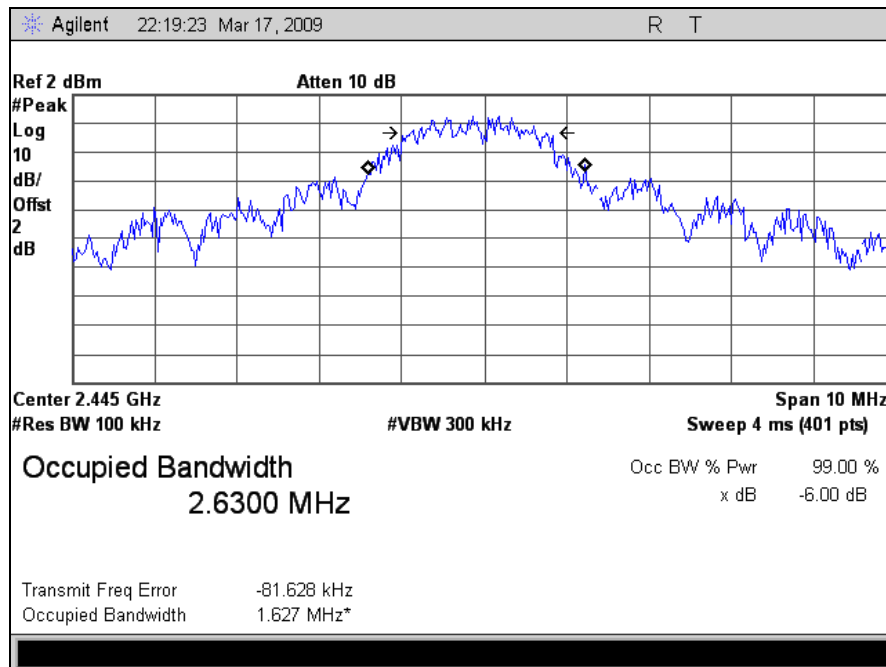
Plot 4. 6 dB Occupied Bandwidth, Mid Channel
