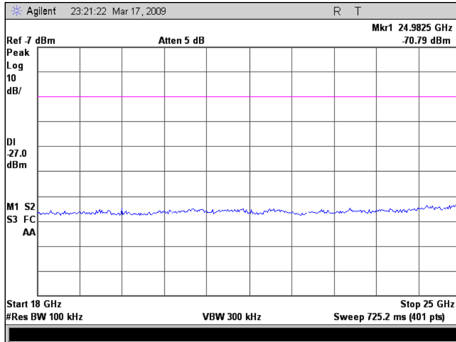
Plot 27. Spurious Conducted Emissions, High Channel, 18 GHz – 25 GHz
