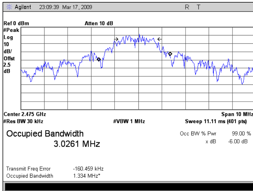
Plot 8. 99% Occupied Bandwidth, High Channel
