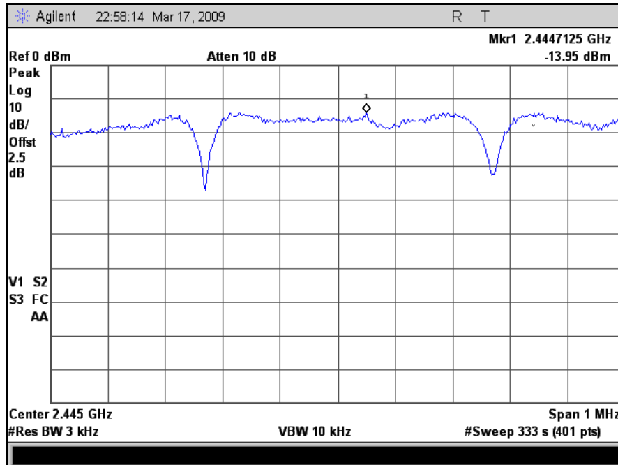
Plot 31. Peak Power Spectral Density, Mid Channel
