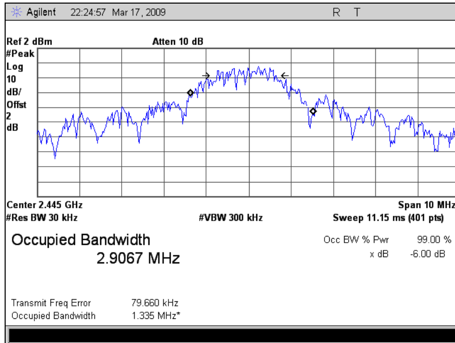
Plot 7. 99% Occupied Bandwidth, Mid Channel
