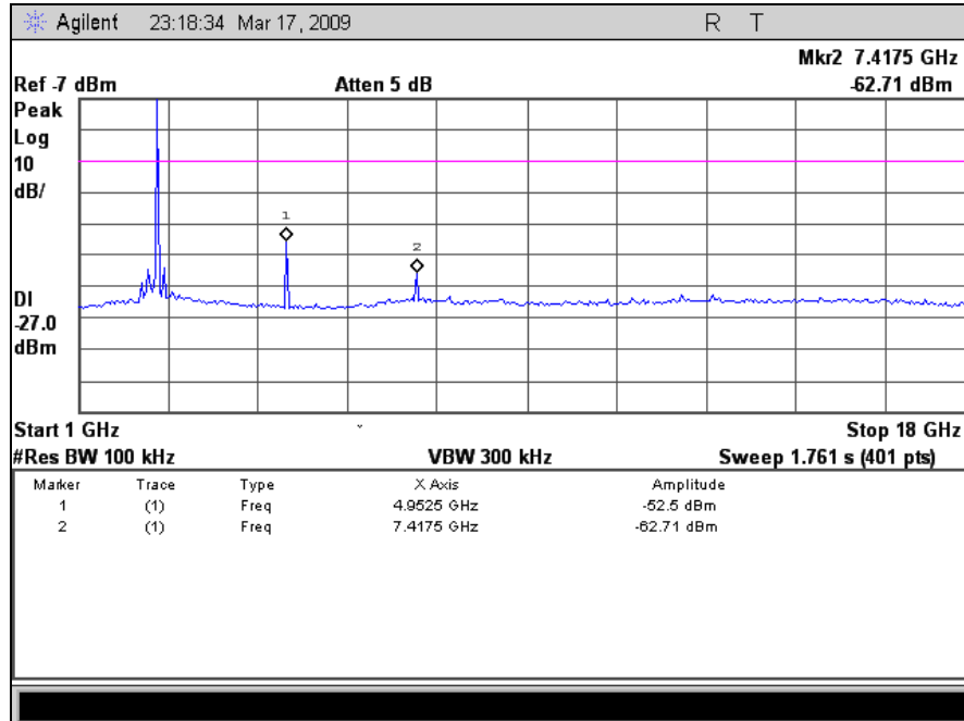
Plot 26. Spurious Conducted Emissions, High Channel, 1 GHz – 18 GHz
