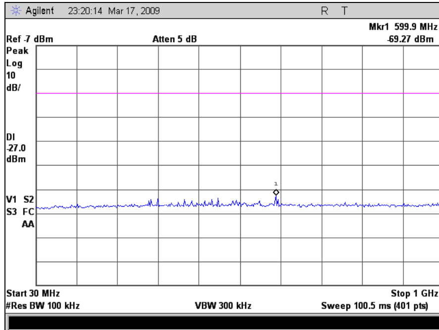
Plot 25. Spurious Conducted Emissions, High Channel, 30 MHz – 1 GHz
