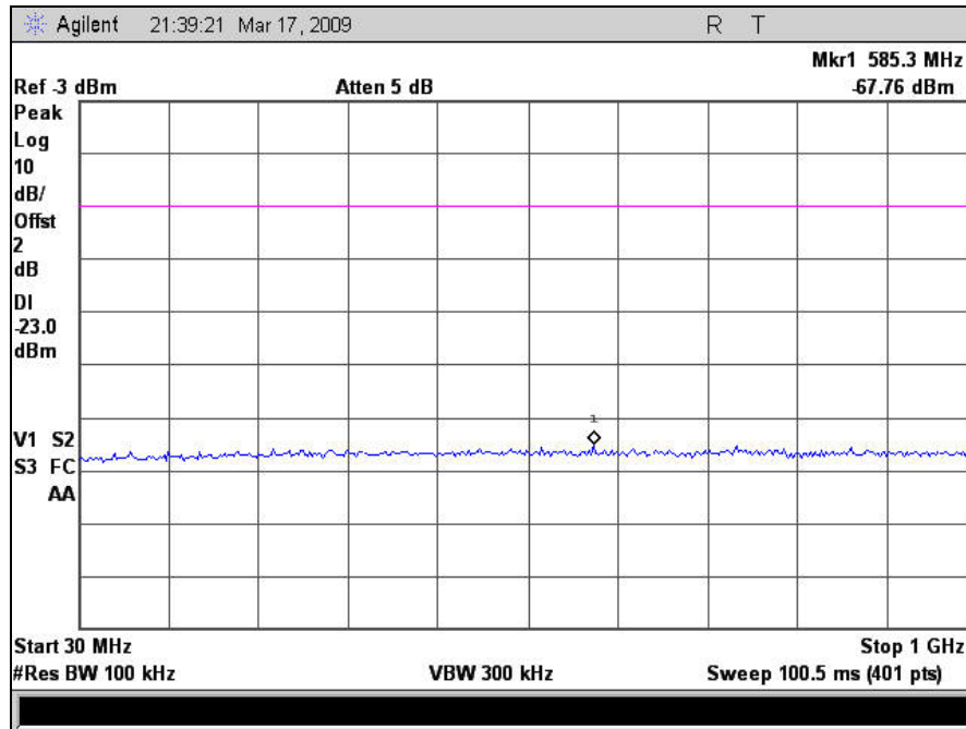
Plot 19. Spurious Conducted Emissions, Low Channel, 30 MHz – 1 GHz
