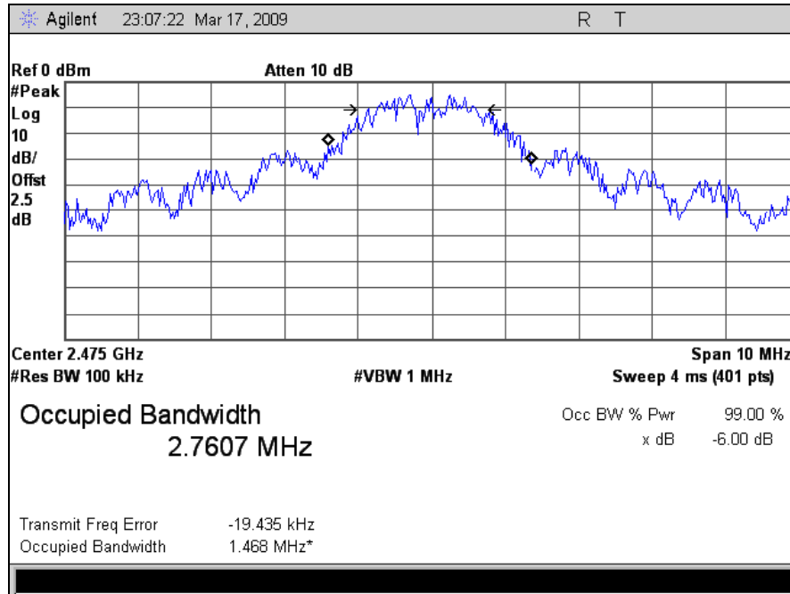
Plot 5. 6 dB Occupied Bandwidth, High Channel
