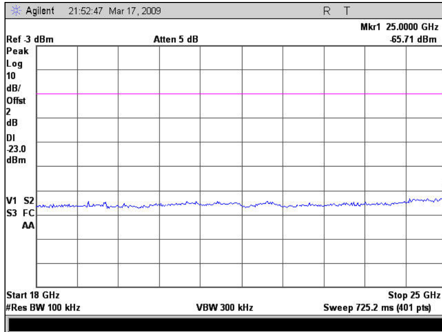
Plot 21. Spurious Conducted Emissions, Low Channel, 18 GHz – 25 GHz
