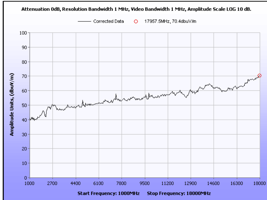
Plot 13. Radiated Harmonic Emissions, Mid Channel
