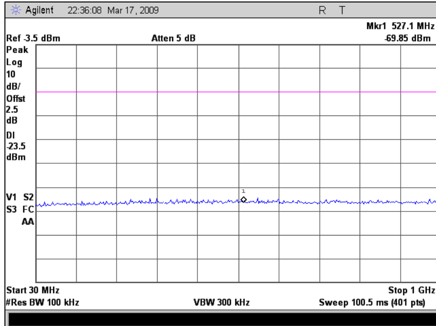
Plot 22. Spurious Conducted Emissions, Mid Channel, 30 MHz – 1 GHz
