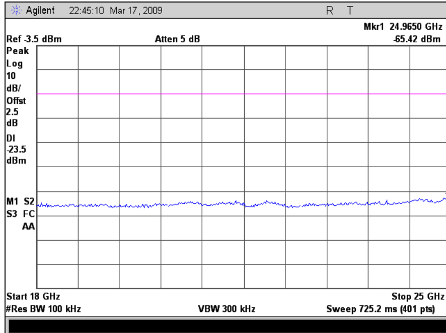
Plot 24. Spurious Conducted Emissions, Mid Channel, 18 GHz – 25 GHz
