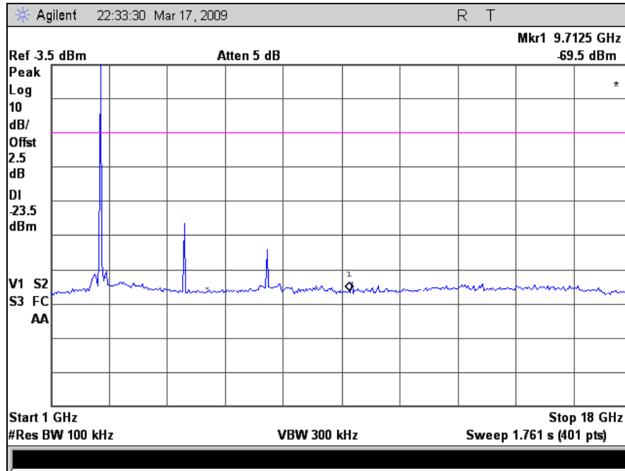
Plot 23. Spurious Conducted Emissions, Mid Channel, 1 GHz – 18 GHz
