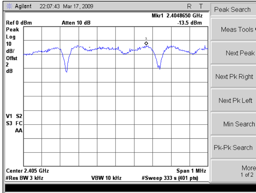
Plot 30. Peak Power Spectral Density, Low Channel
