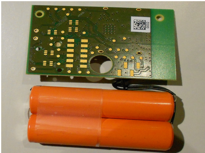
PCB backside, identical for all models:
