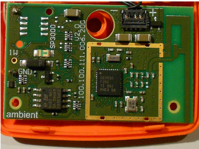
PCB front-side SP3000T, SP3000T1W and SP3000TERS:
