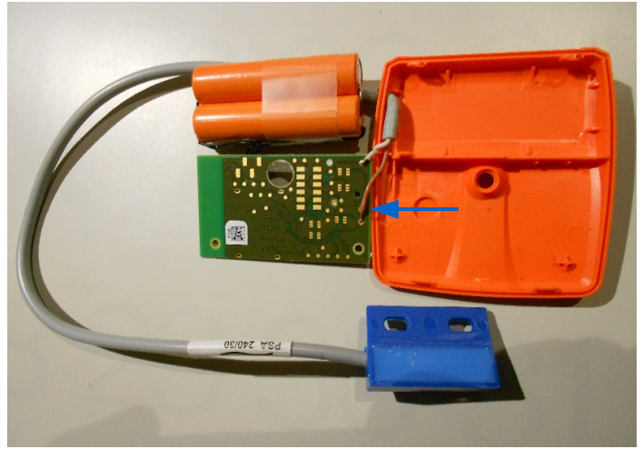
SP3000TERS, connection of external Reed sensor cable:
