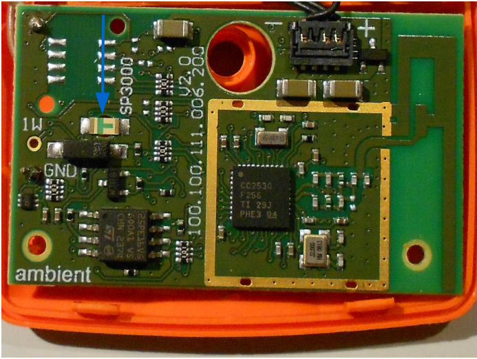
Position of temperature sensor, for all models:
