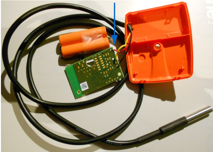
SP3000T1W, connection of external 1W sensor cable:
