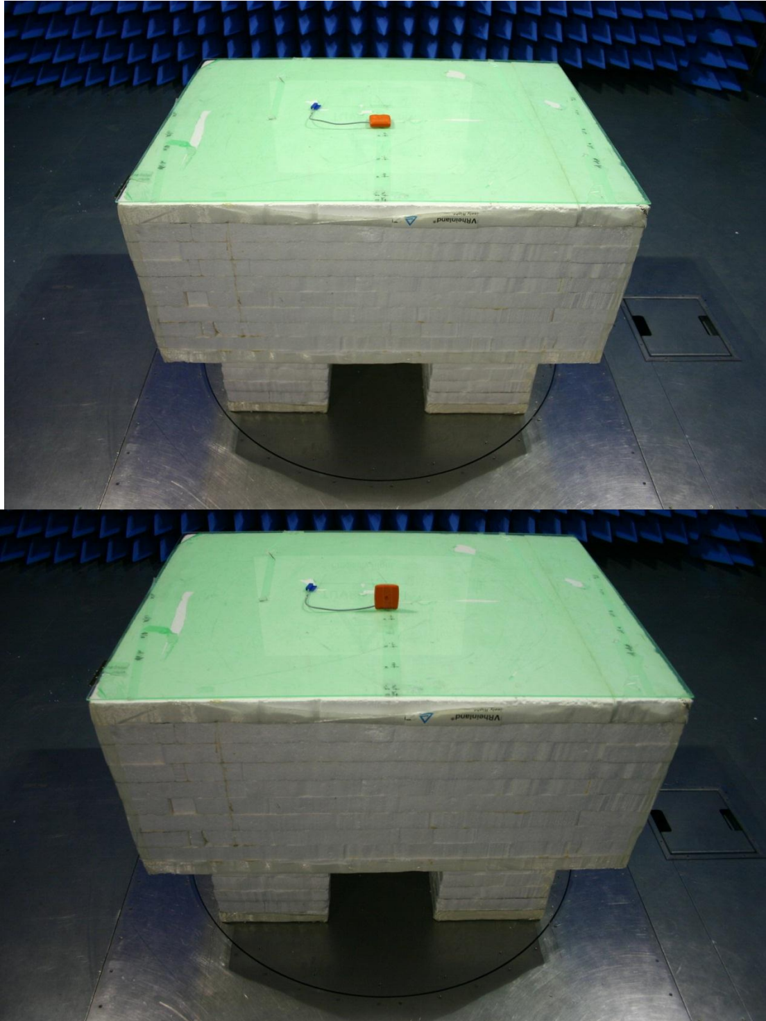
Model SP3000TERS with Reed contacts, placed horizontal and vertical
