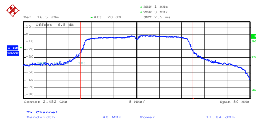
Middle channel
