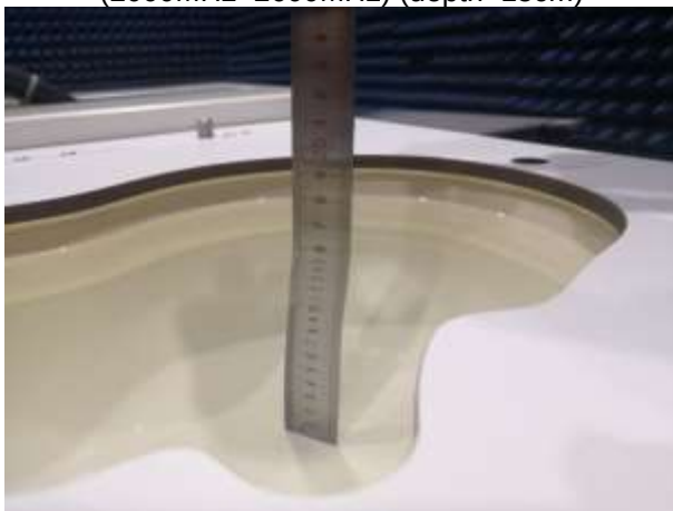
Fig. 9.7 Photo of Liquid Height for Head SAR (5000MHz~6000MHz) (depth>15cm)
