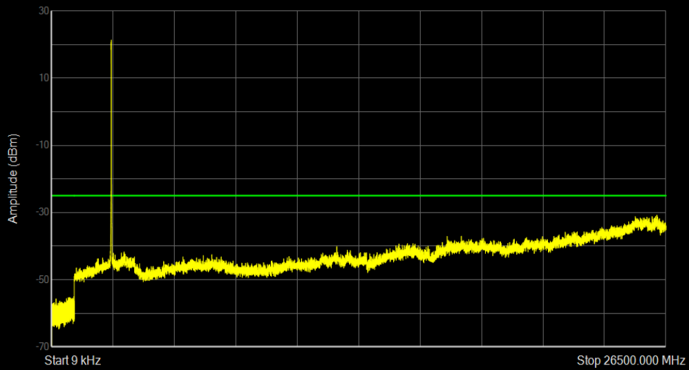
Band41 QAM16 BW=10MHz Channel=40620 RB Size=50 Position=#0
