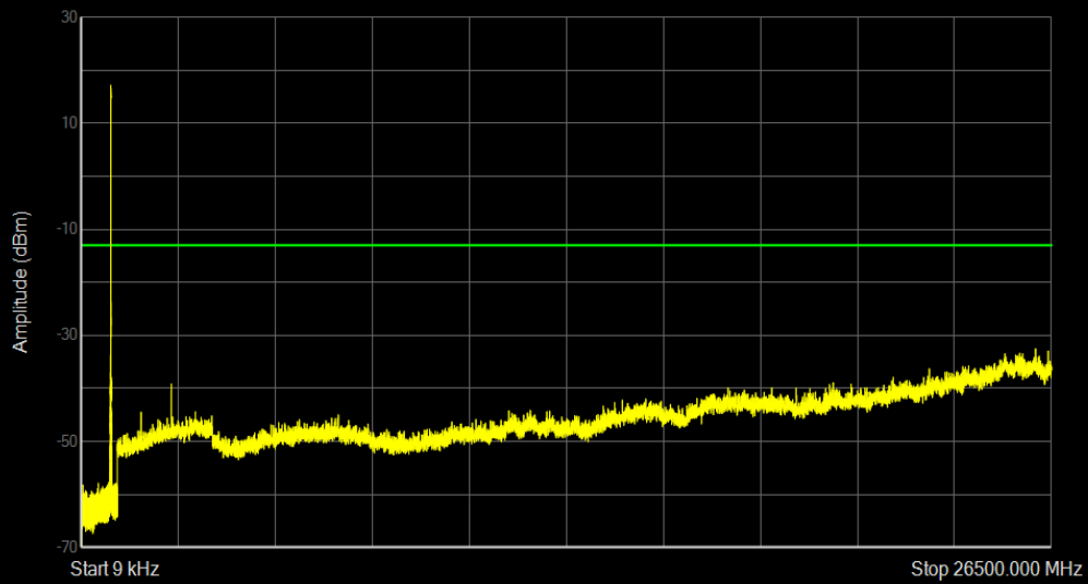
Band26(824-849) QPSK BW=3MHz Channel=26805 RB Size=15 Position=#0
