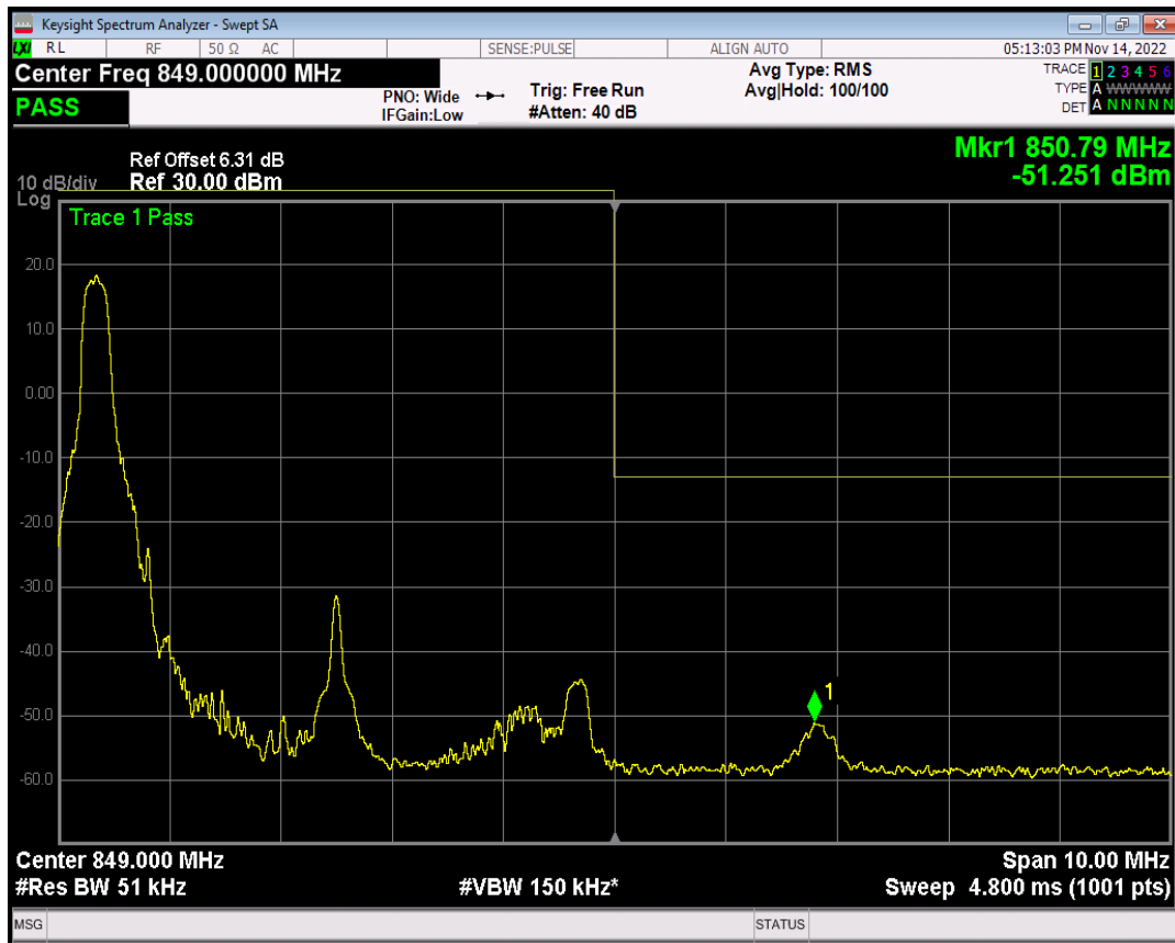
Band26(824-849) QAM16 BW=5MHz Channel=27015 RB Size=1 Position=#Max
