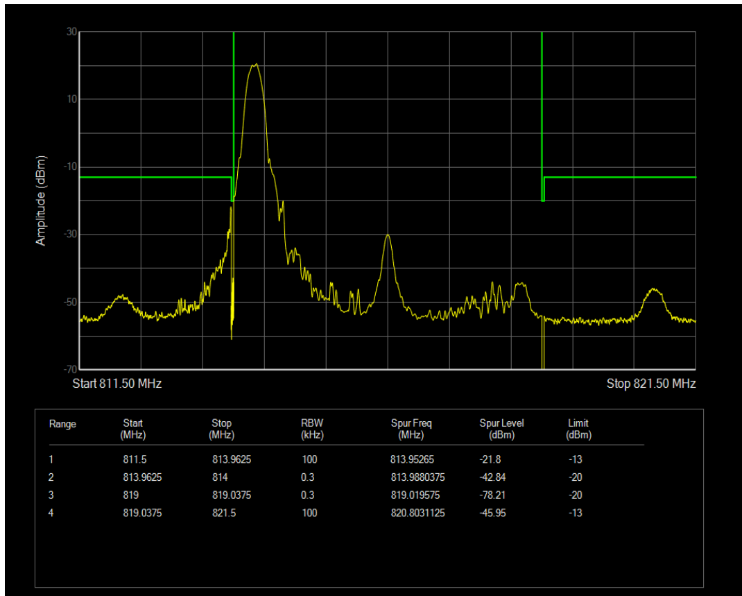
Band26(814-824) QAM16 BW=5MHz Channel=26715 RB Size=1 Position=#Max
