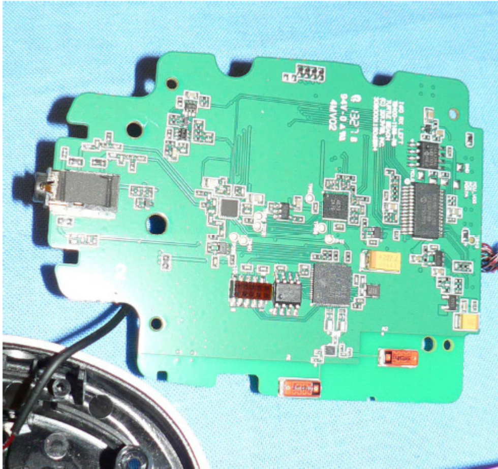
Wifi Board
