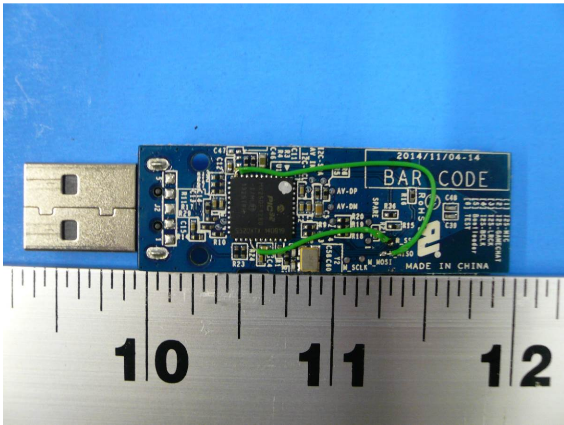
Figure 2: Internal Photo of Ear Force Stealth 450 TX - Bottom
