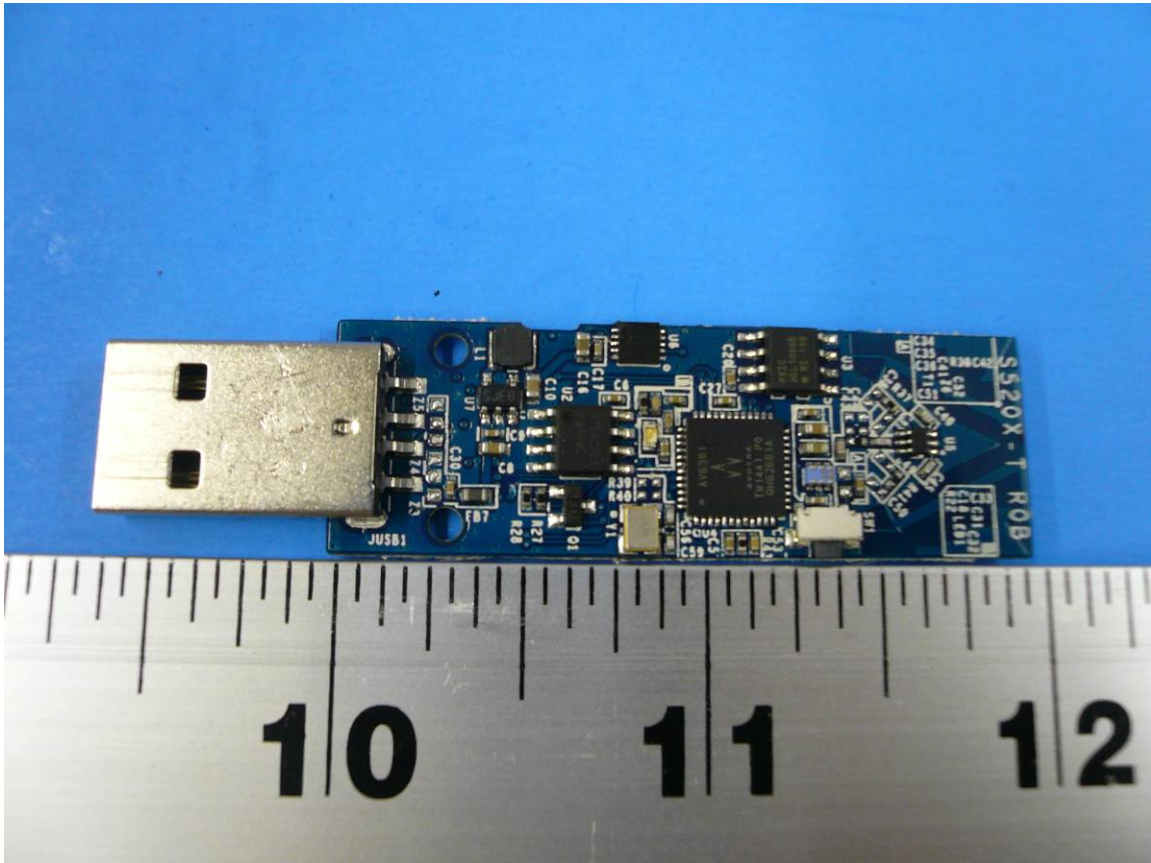
Figure 1: Internal Photo of Ear Force Stealth 450 TX - Top
