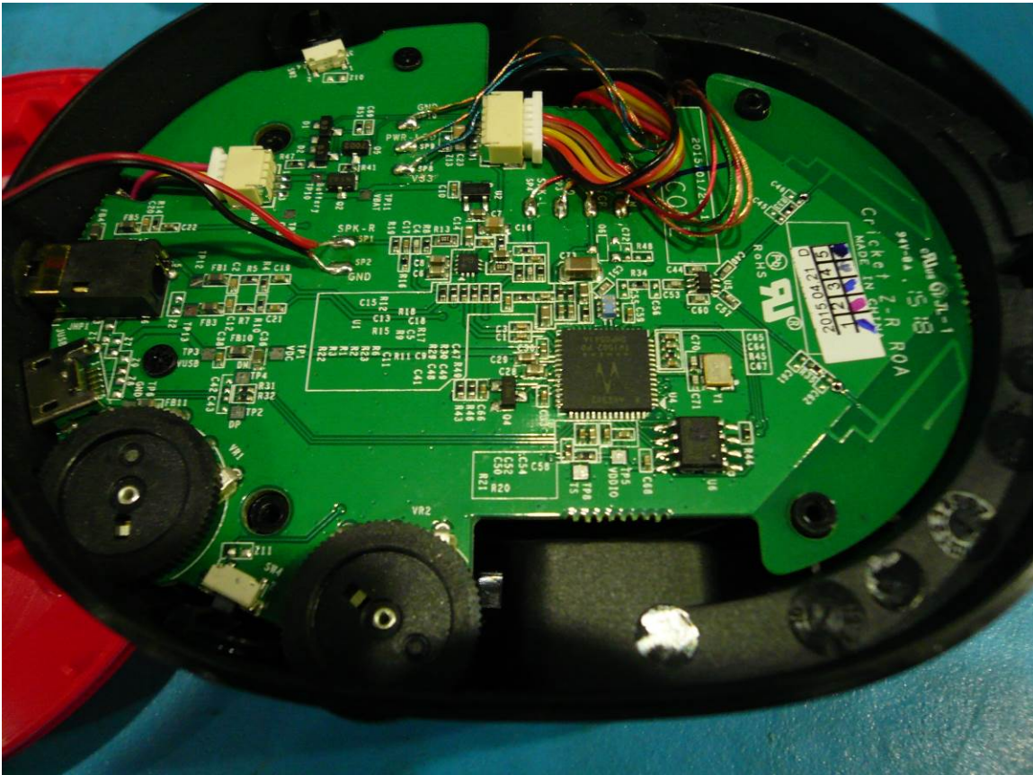
Figure 1: Internal Photo of Ear Force Stealth 450 RX - Top
