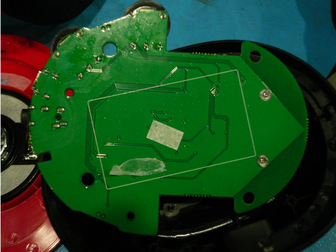
Figure 3: Internal Photo of Ear Force Stealth 450 RX without battery- Bottom
