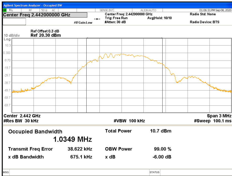
Figure 9: 99% Bandwidth-Transmitter -2442 MHz
