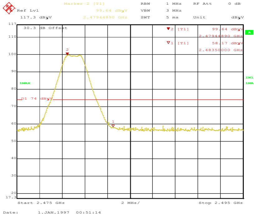
Figure 24: Band-edge-2480 MHz-V-Pk
