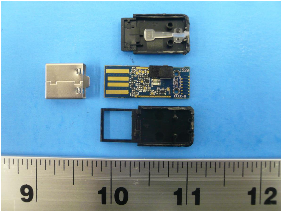
Figure 1: Internal Photo of Stealth 700P Gen 2 TX with Plastic Cover Removed
