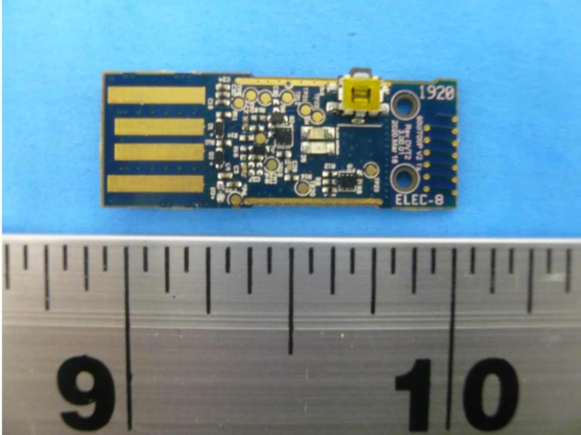
Figure 2: Internal Photo of Stealth 700P Gen 2 TX – Top PCB
