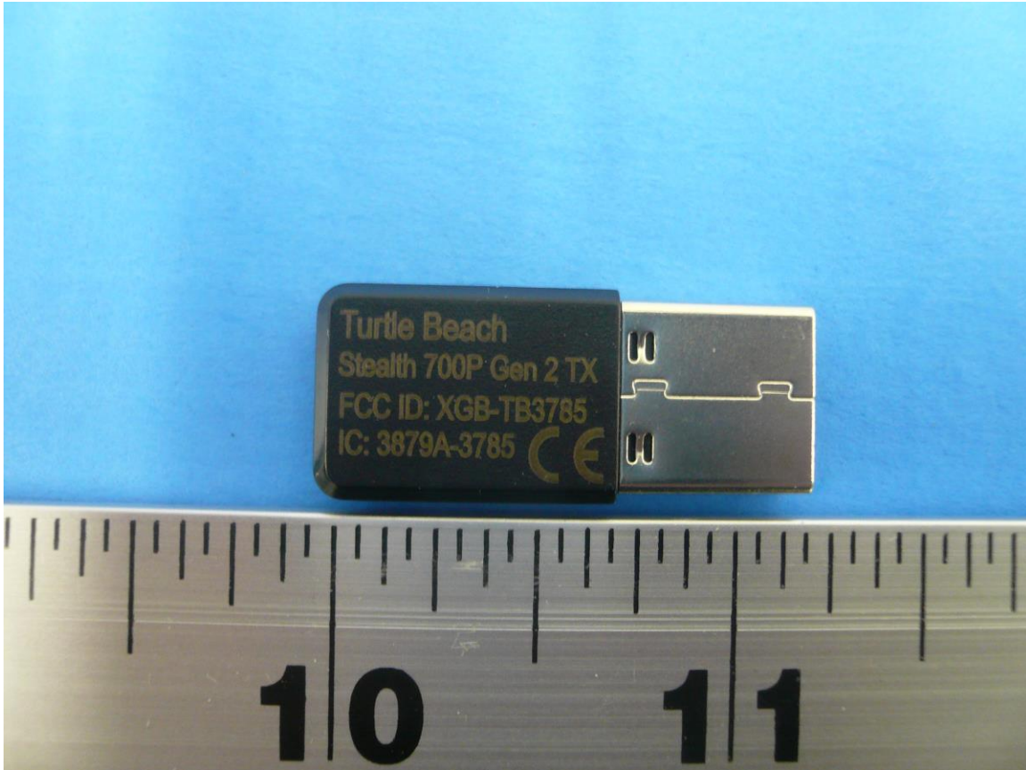
Figure 2: External Photo of Stealth 700P Gen 2 TX - Bottom
