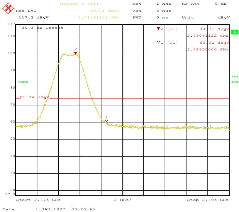
Figure 24: Band-edge-2480 MHz-V-Pk
