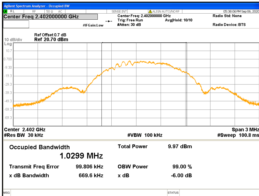
Figure 8: 99% Bandwidth-Headset -2402 MHz
