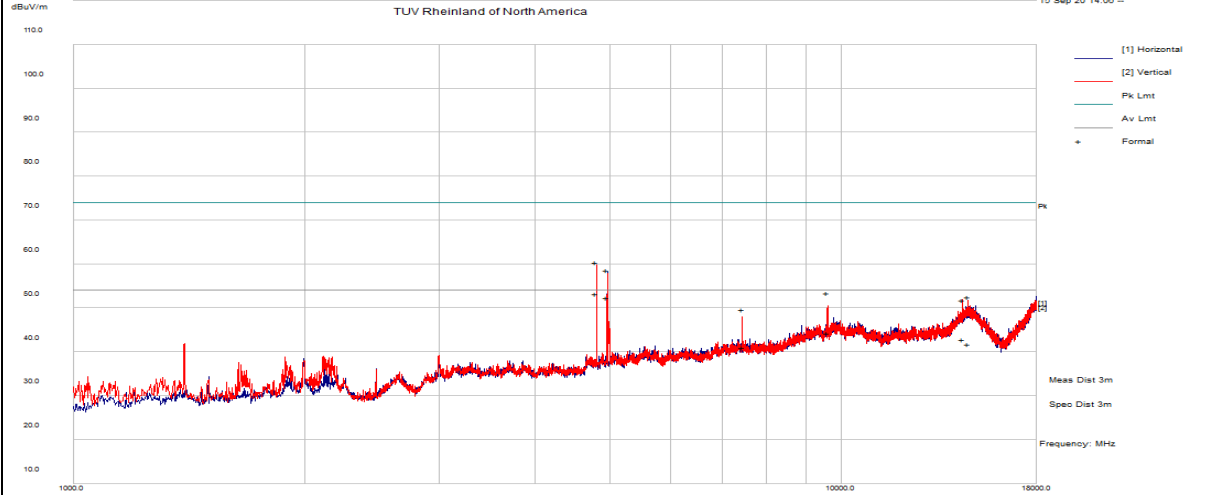
Turtle Beach, Stealth 700P Gen 2 RX, Collocation: NXP Radios TX @ 2402MHz and BLE Radio TX @ 2480 (The highest powers of both radios) Filename: c:\program files (x86)\emisoft - vasona\results\TB-20200915-RE3.emi
