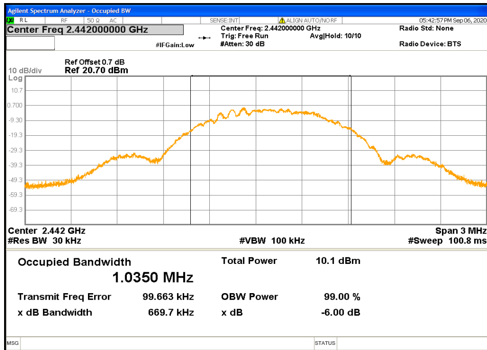
Figure 9: 99% Bandwidth-Headset -2442 MHz
