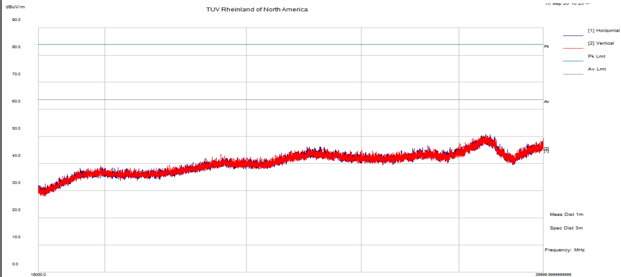
Turtle Beach, Stealth 700P Gen 2 RX, Collocation: NXP Radios TX @ 2402MHz and BLE Radio TX @ 2480 (The highest powers of both radios) Filename: c:\program files (x86)\emisoft - vasona\results\TB-20200915-RE5.emi
