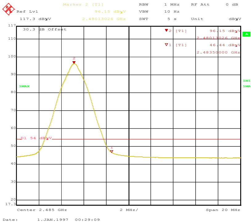
Figure 25: Band-edge-2480 MHz-V-Ave
