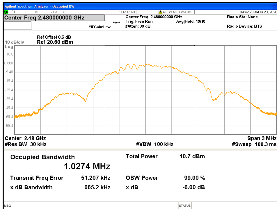
Figure 10: 99% Bandwidth-Headset -2480 MHz
