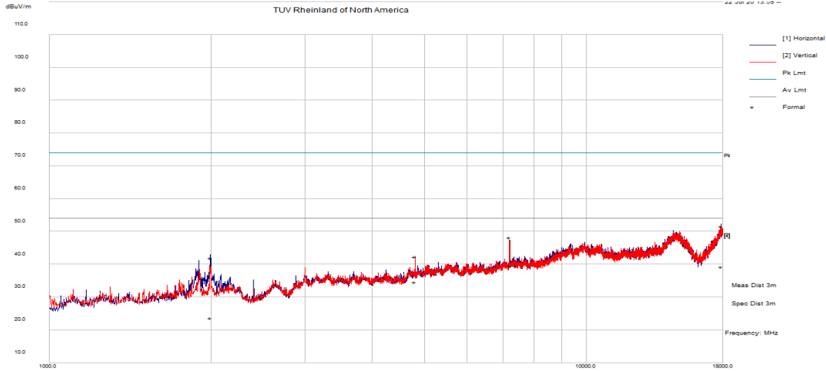
Above 1GHz Plots for Transmit Mode at 2402 MHz
