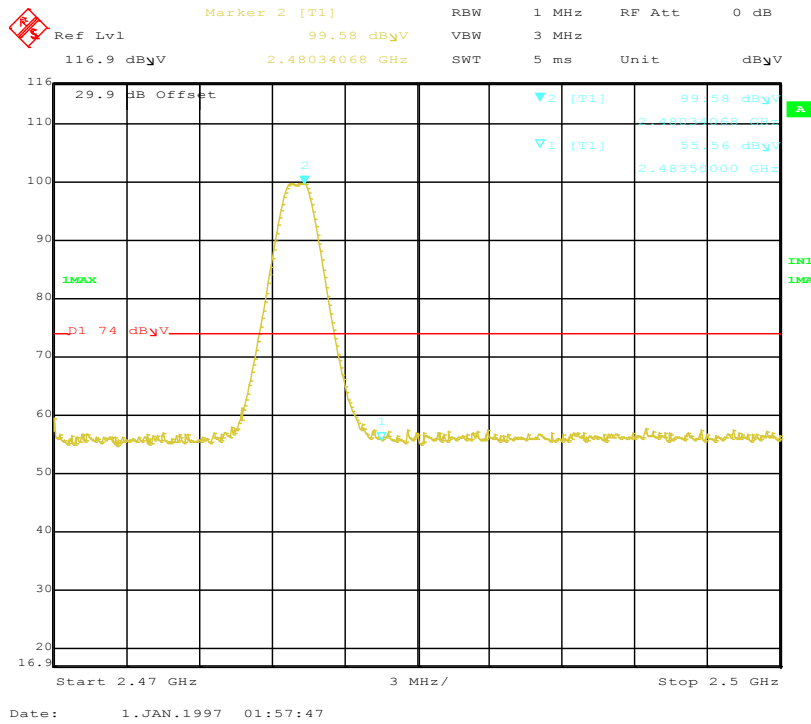
Figure 26: Band-edge-2480 MHz-H-Pk
