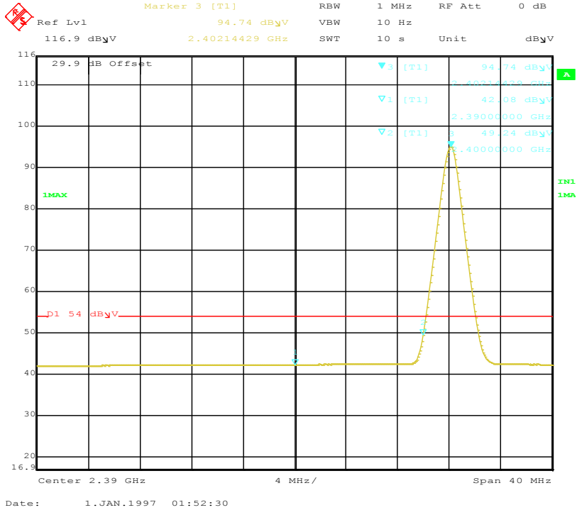
Figure 23: Band-edge-2402 MHz-H-Ave
