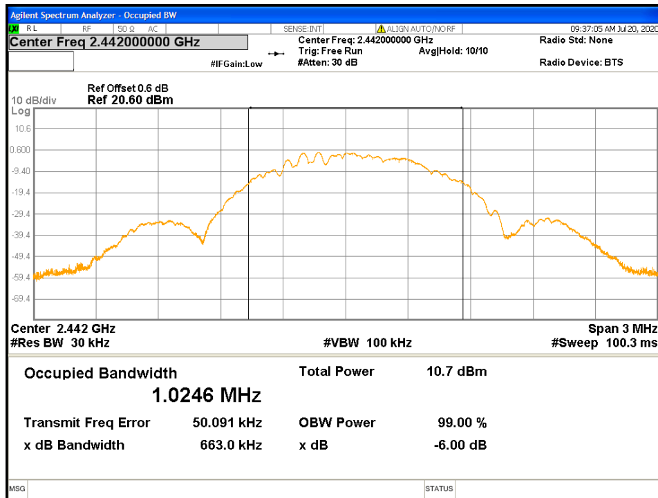
Figure 9: 99% Bandwidth-Headset -2442 MHz
