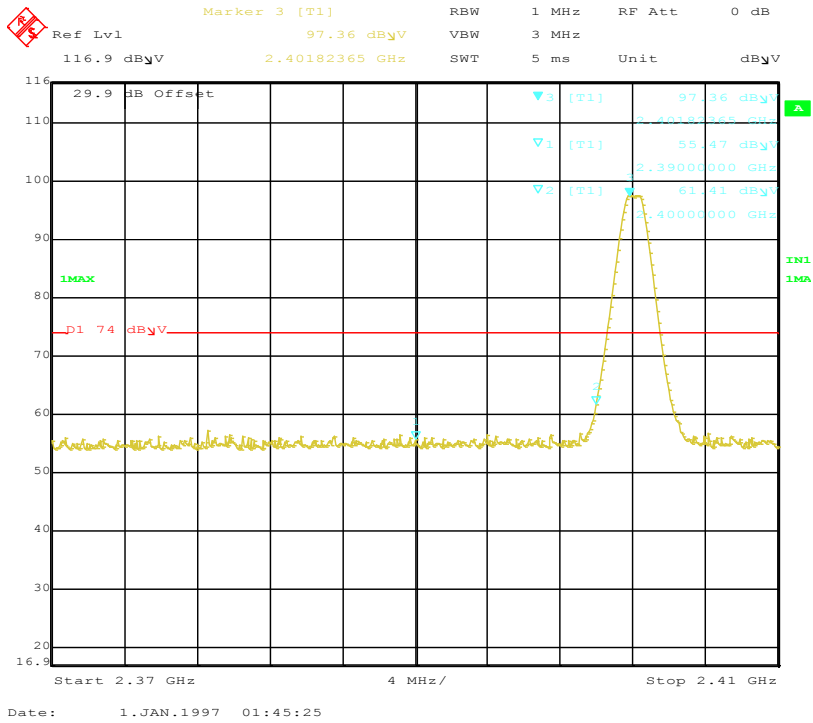
Figure 20: Band-edge-2402 MHz-V-Pk
