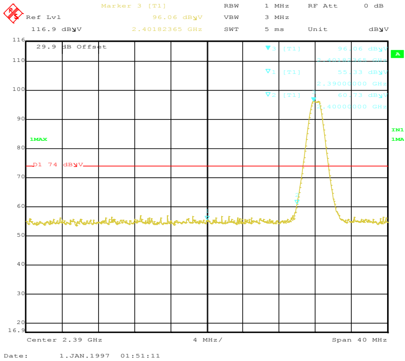
Figure 22: Band-edge-2402 MHz-H-Pk
