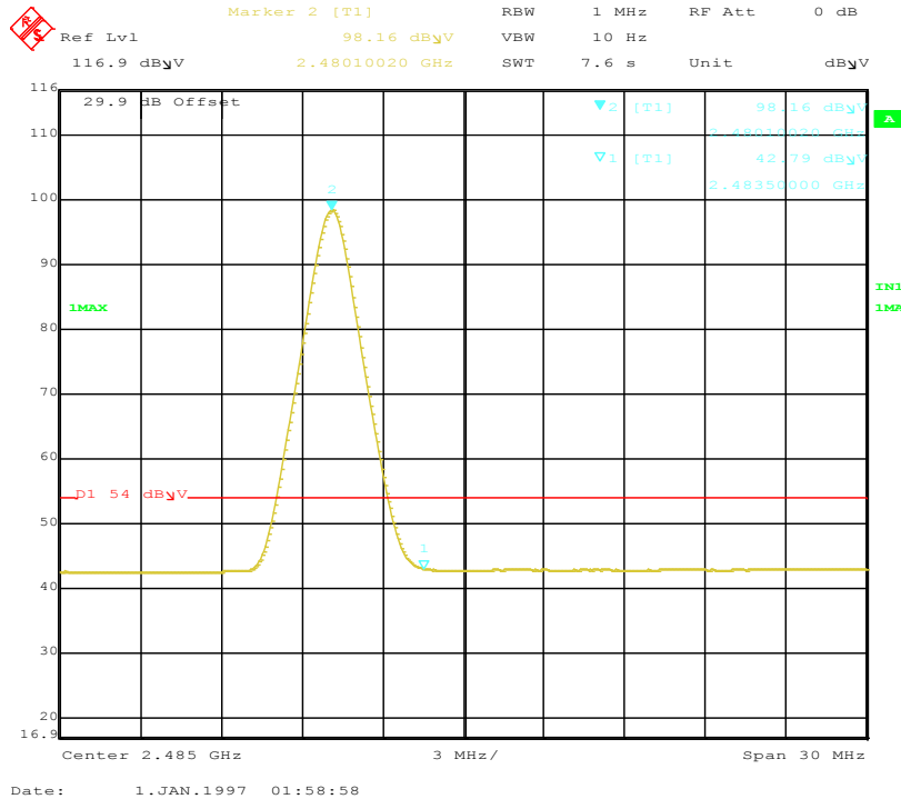
Figure 27: Band-edge-2480 MHz-H-Ave
