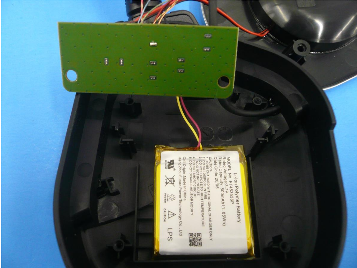
Figure 5: Internal Photo of Stealth 700P Gen 2 RX – Right Ear PCB (Bottom)
