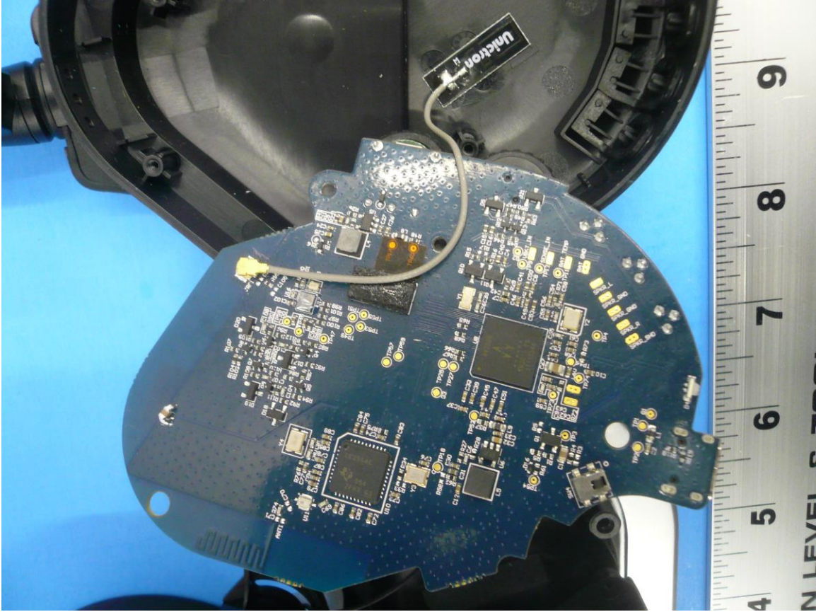
Figure 3: Internal Photo of Stealth 700P Gen 2 RX – Main PCB (Bottom)
