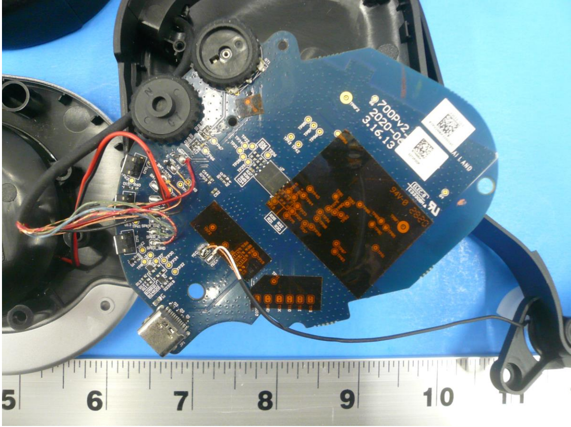
Figure 2: Internal Photo of Stealth 700P Gen 2 RX – Main PCB (Top)
