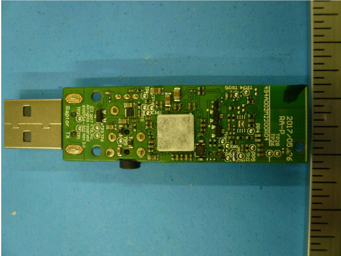
Figure 2: Internal Photo of Ear Force Stealth 700P TX - Bottom
