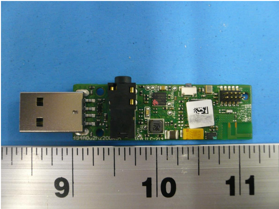
Figure 1: Internal Photo of Ear Force Stealth 700P TX - Top
