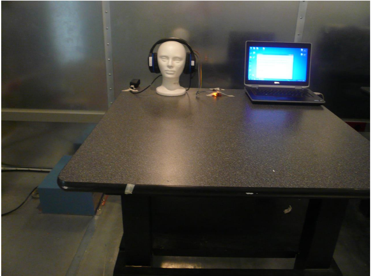
Figure 9: AC Conducted Emission Test Setup (Front)
