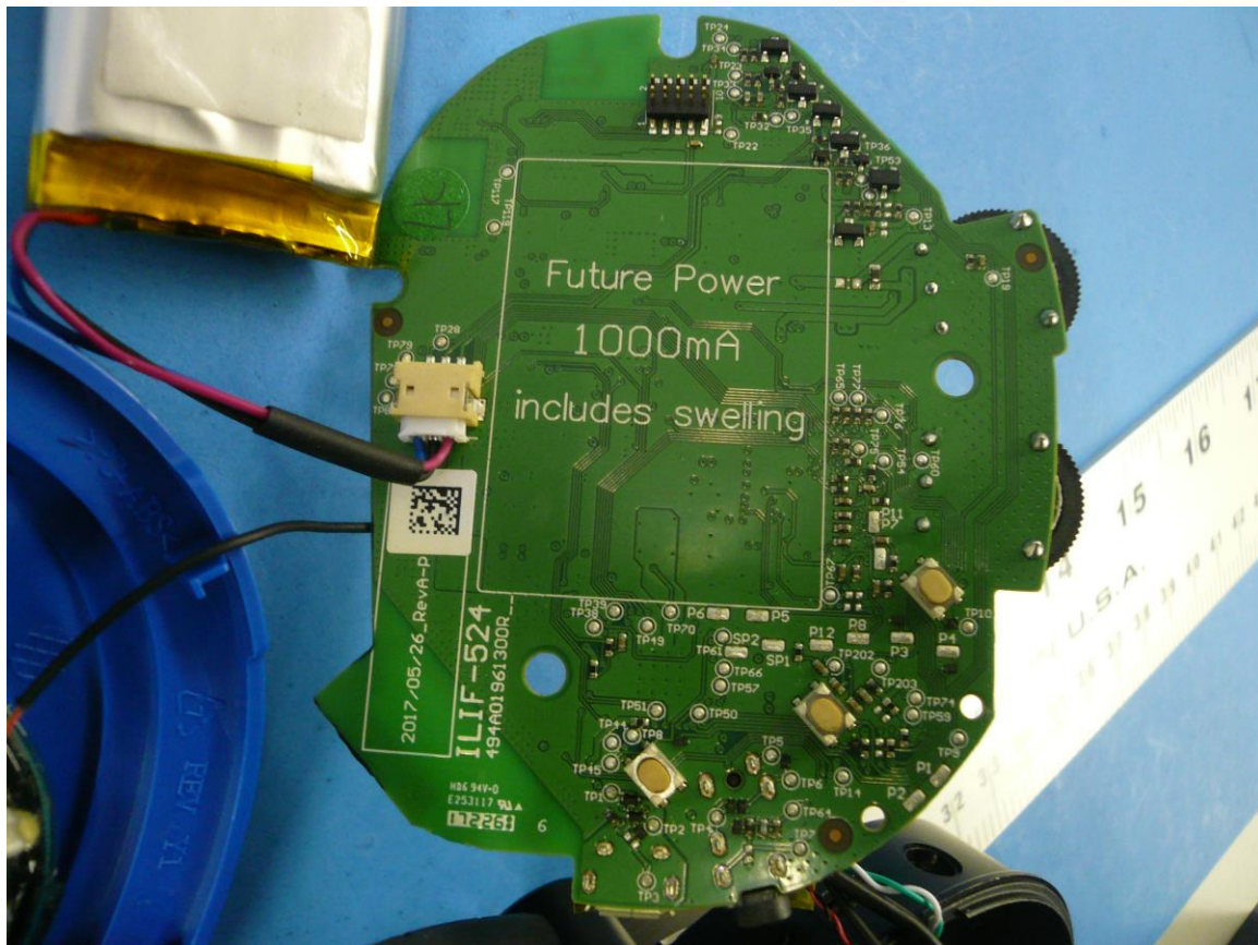
Figure 5: Internal Photo of Ear Force Stealth 700P RX PCB (Bottom without Battery)
