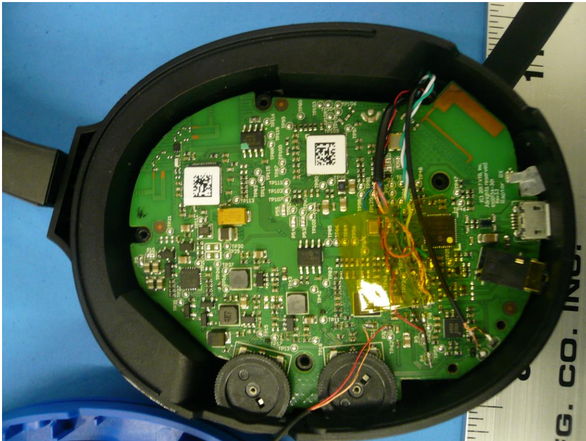
Figure 3: Internal Photo of Ear Force Stealth 700P RX PCB (Top)
