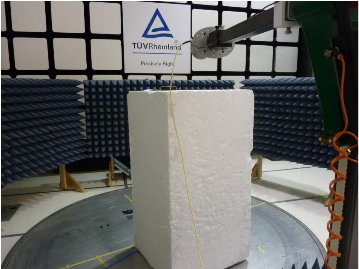
Figure 5: Test Setup for 18 GHz to 40GHz (Front View)
