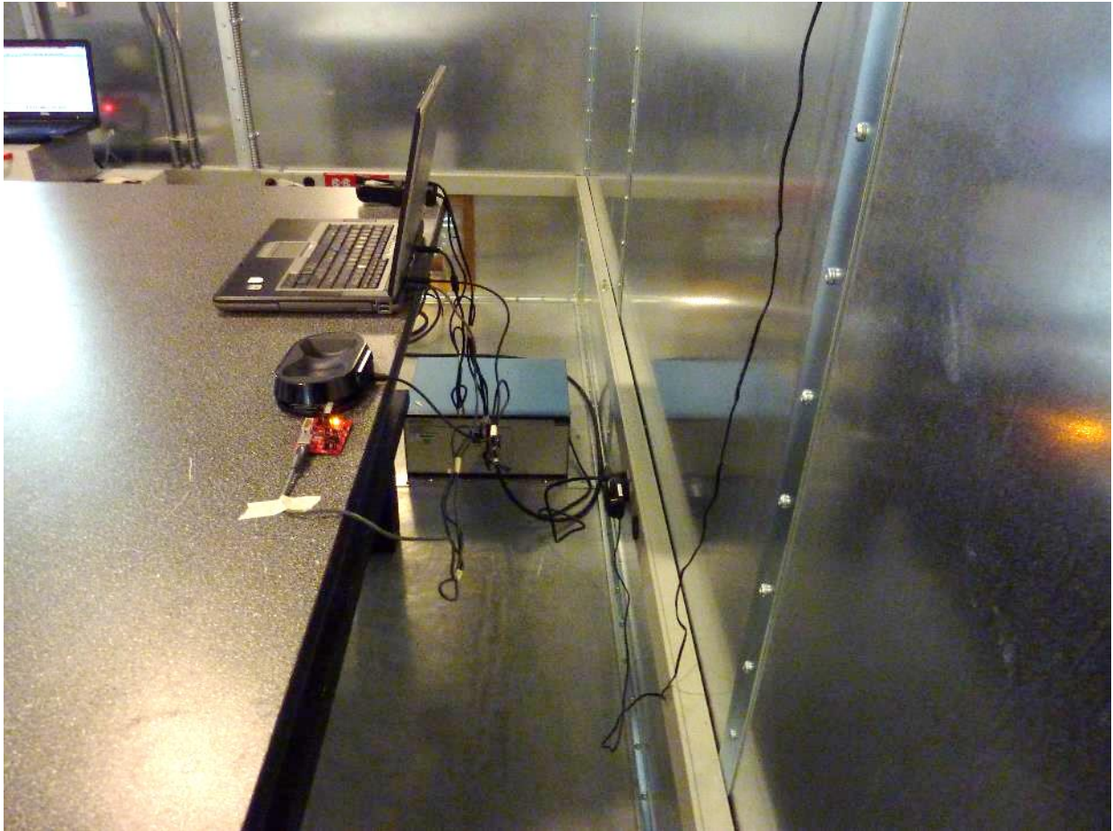
Figure 12: Conducted Emissions Test Setup (Side View)
