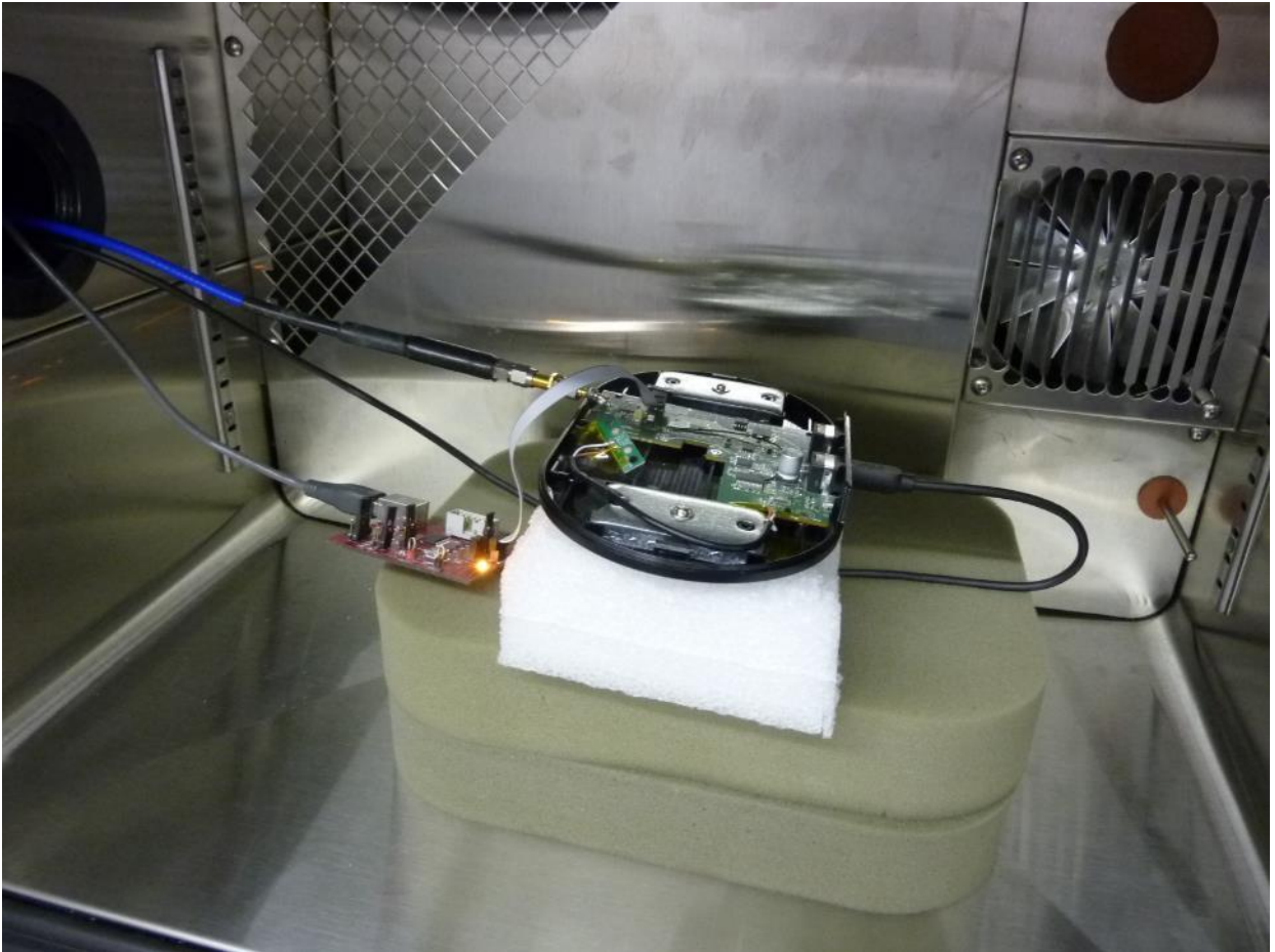
Figure 10: Frequency Stability Test Setup (Inside Thermo Chamber)
