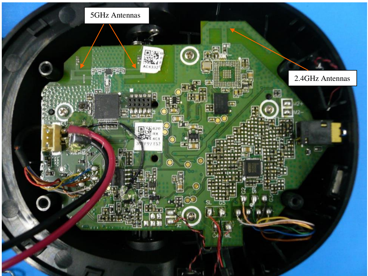
Figure 3: Internal Photo of Elite 800 RX – Antenna Location
