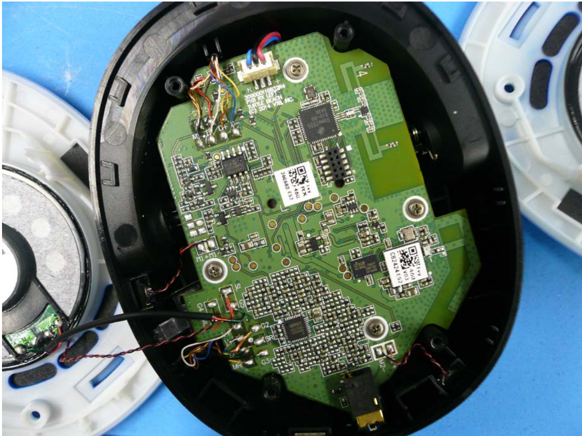
Figure 1: Internal Photo of Elite 800 RX – Top
