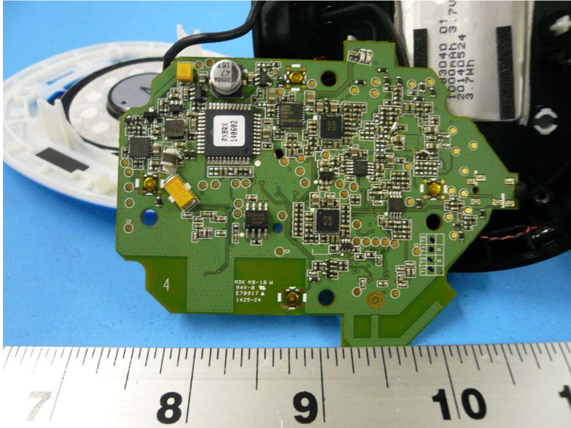
Figure 2: Internal Photo of Elite 800 RX - Bottom
