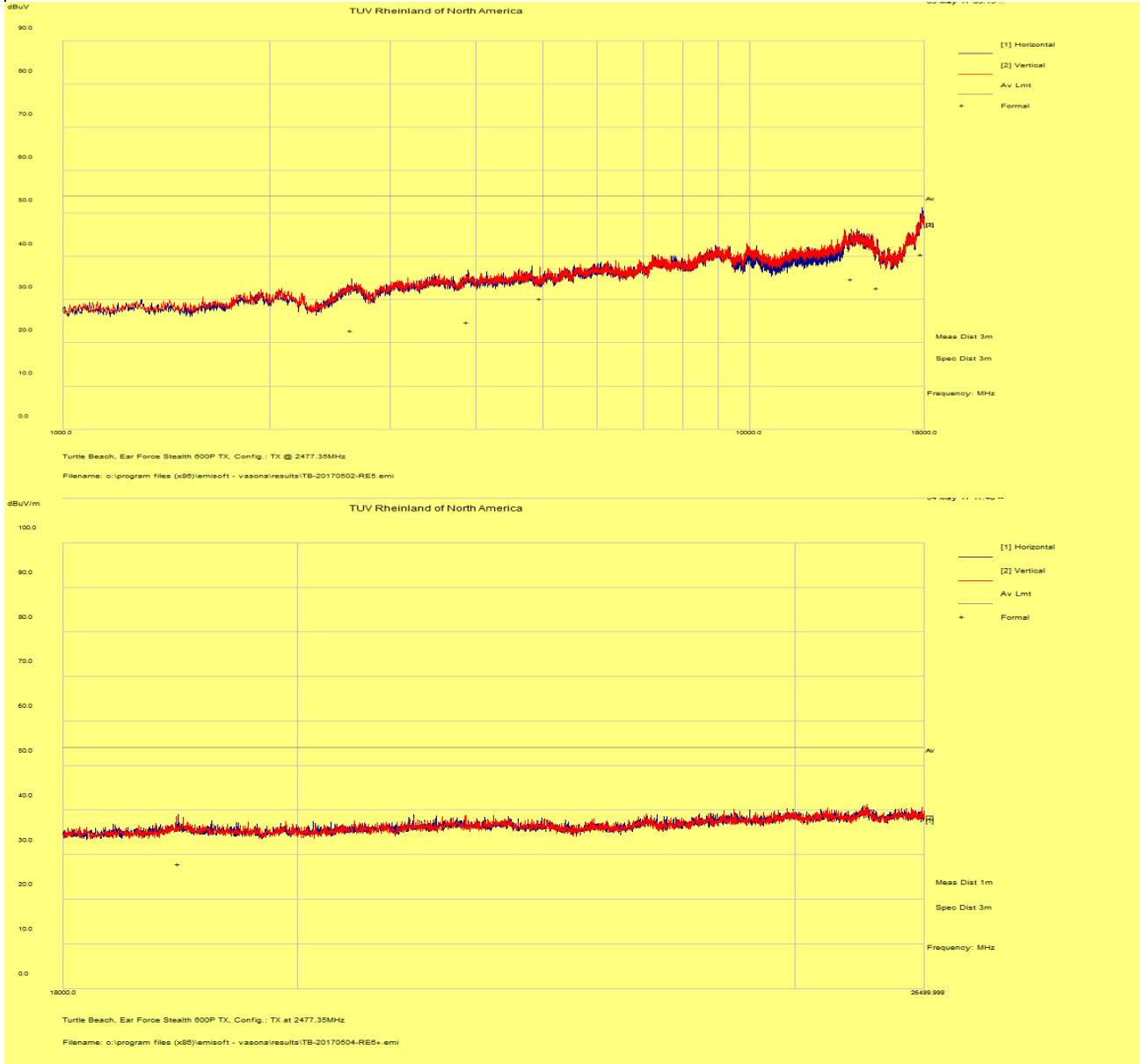
Above 1 GHz Plots for Transmit Mode at 2477.35 MHz
