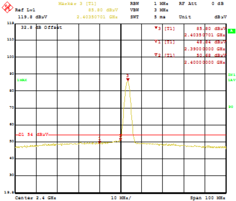
Figure 23: Bandedge-2403.35 MHz-V-Ave
