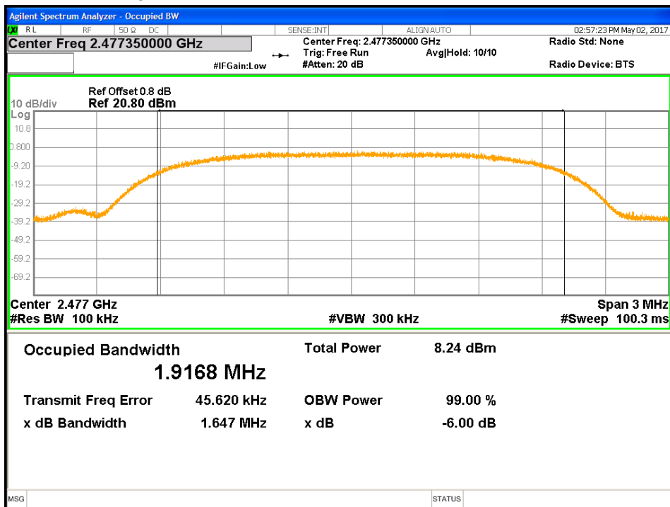
Figure 10: 99% Bandwidth-Transmitter -2477.35 MHz
