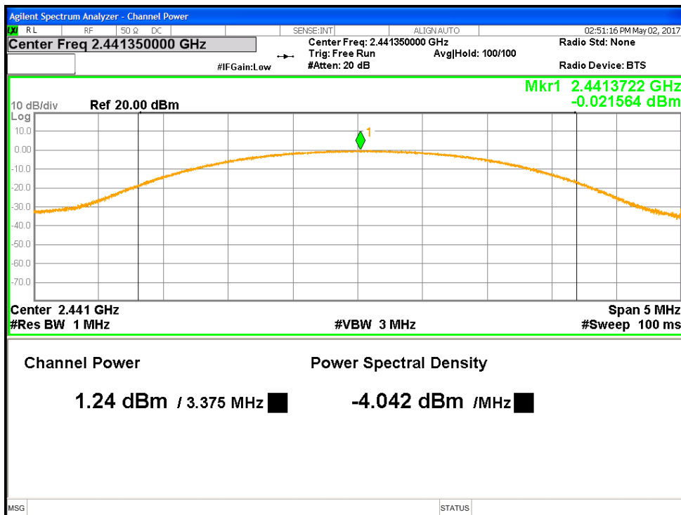
Figure 3: Maximum Conducted Output Power at 2441.35 MHz - USB Transmitter
