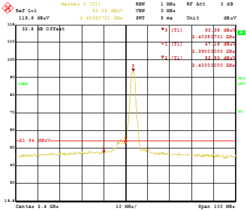
Figure 21: Bandedge-2403.35 MHz-H-Ave
