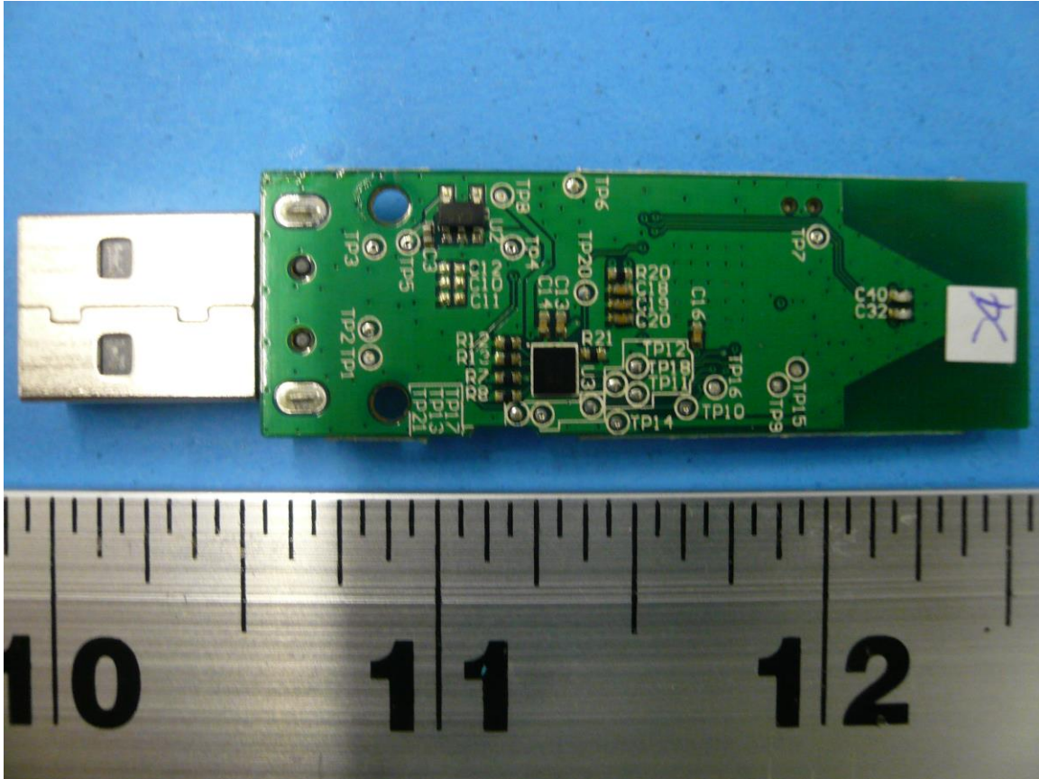
Figure 2: Internal Photo of Ear Force Stealth 600P TX - Bottom
