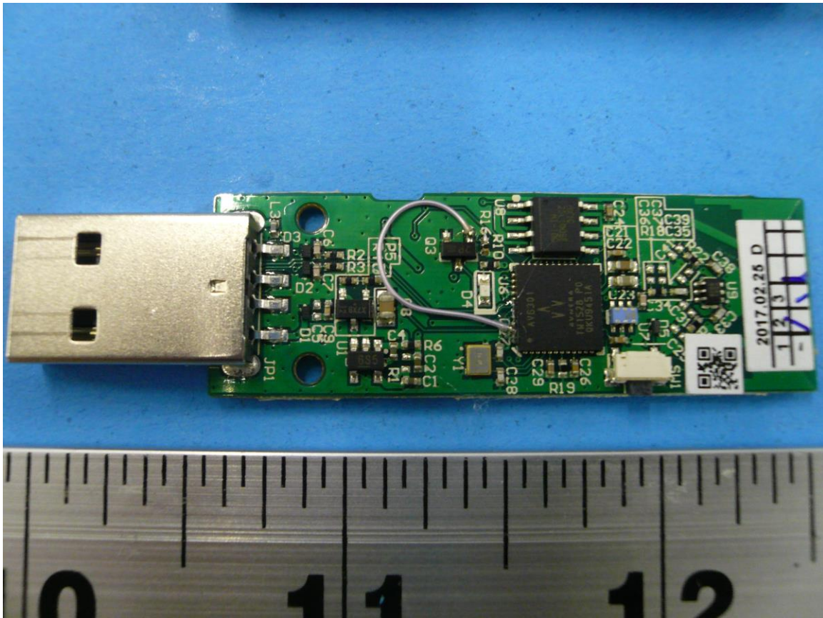
Figure 1: Internal Photo of Ear Force Stealth 600P TX - Top
