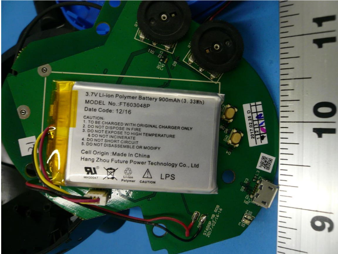
Figure 2: Internal Photo of Ear Force Stealth 600P RX - Bottom
