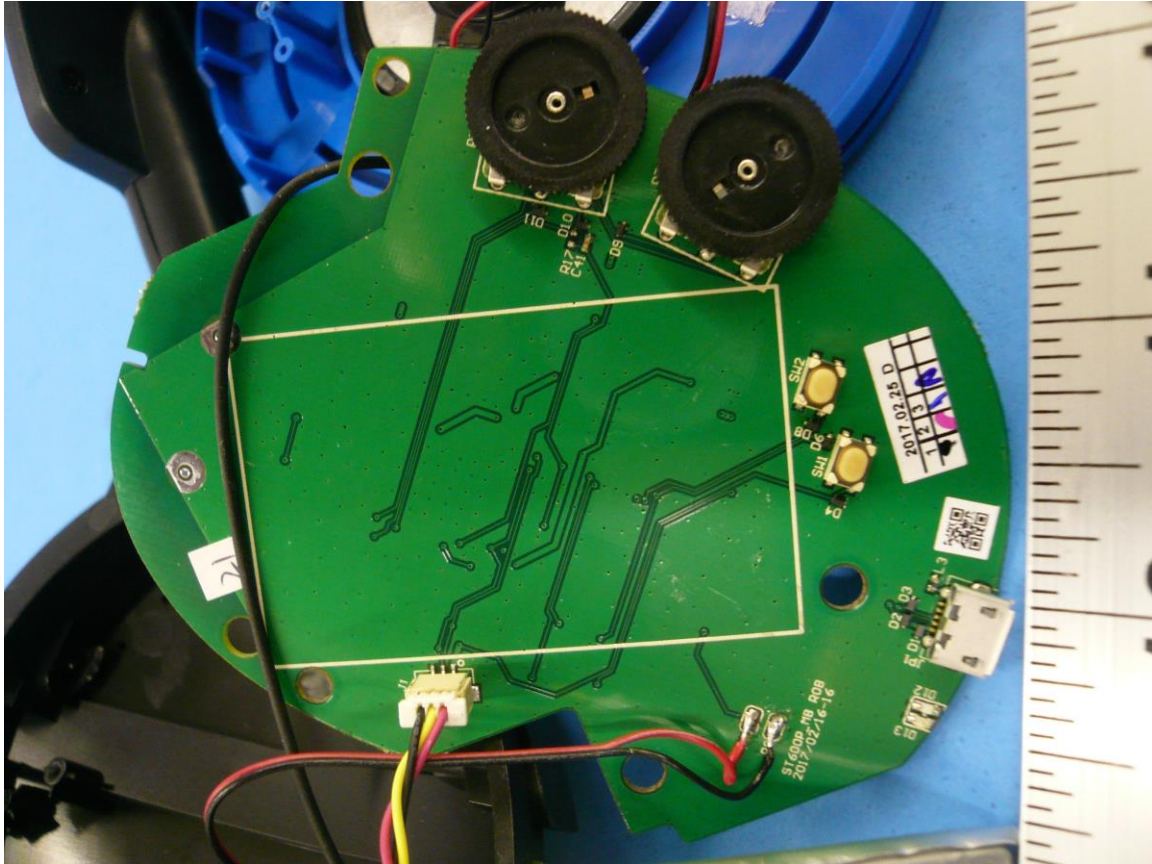
Figure 3: Internal Photo of Ear Force Stealth 600P RX without battery- Bottom
