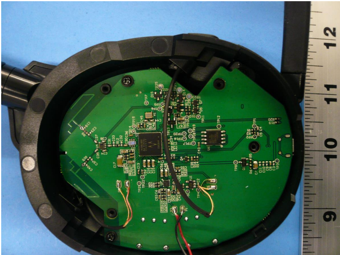
Figure 1: Internal Photo of Ear Force Stealth 600P RX - Top
