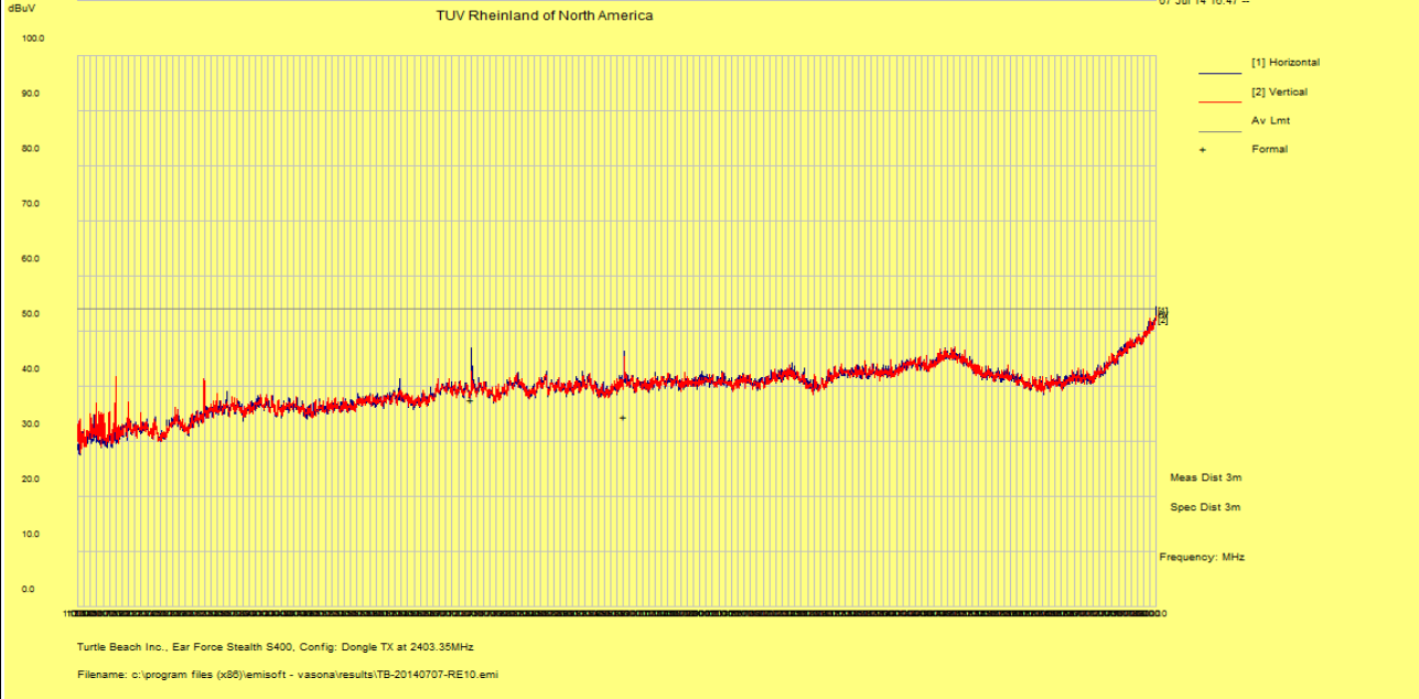
Above 1GHz Plots for Transmit Mode at 2403.35MHz
