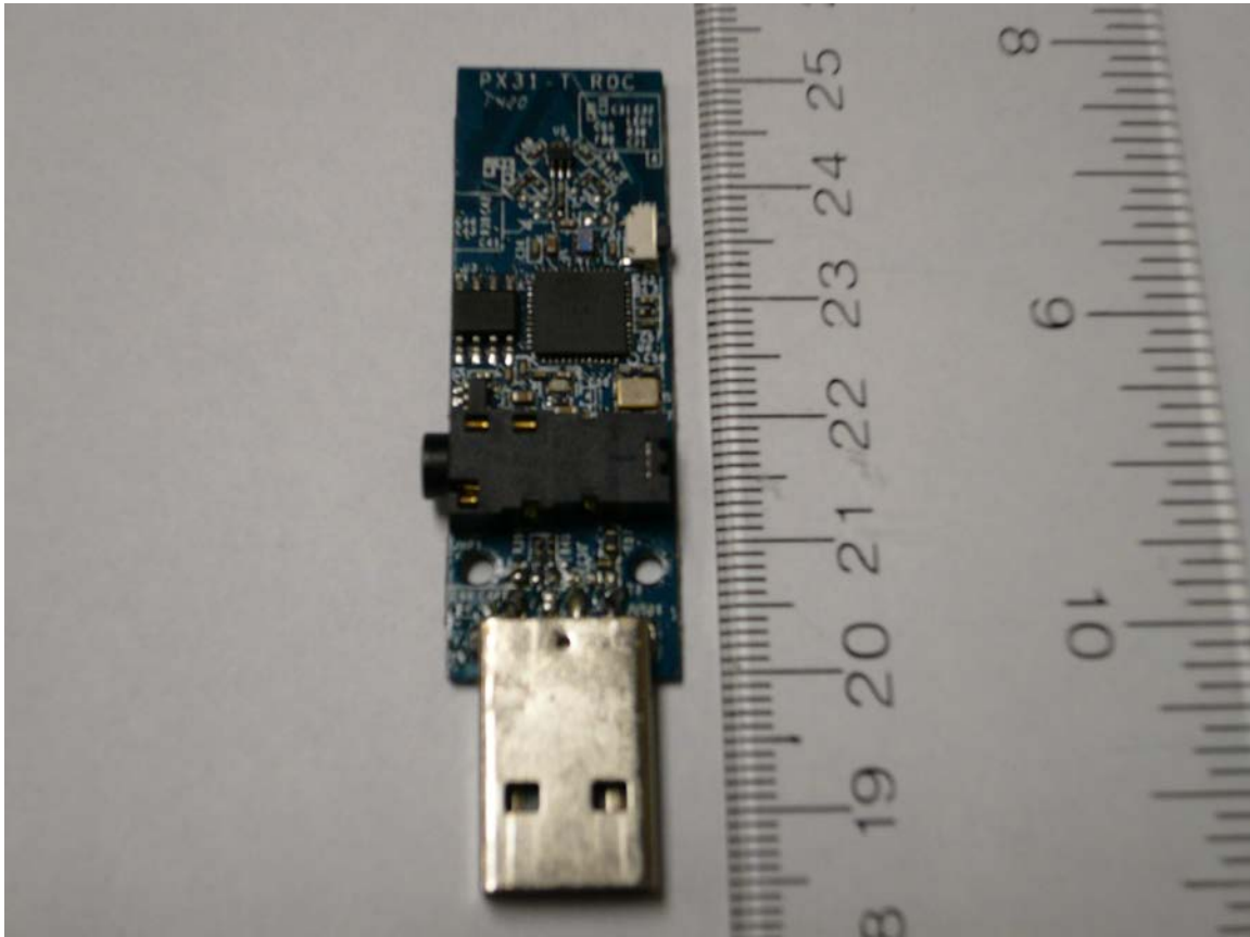
Figure 1: Internal Photo of Ear Force Stealth 500P TX - Top
