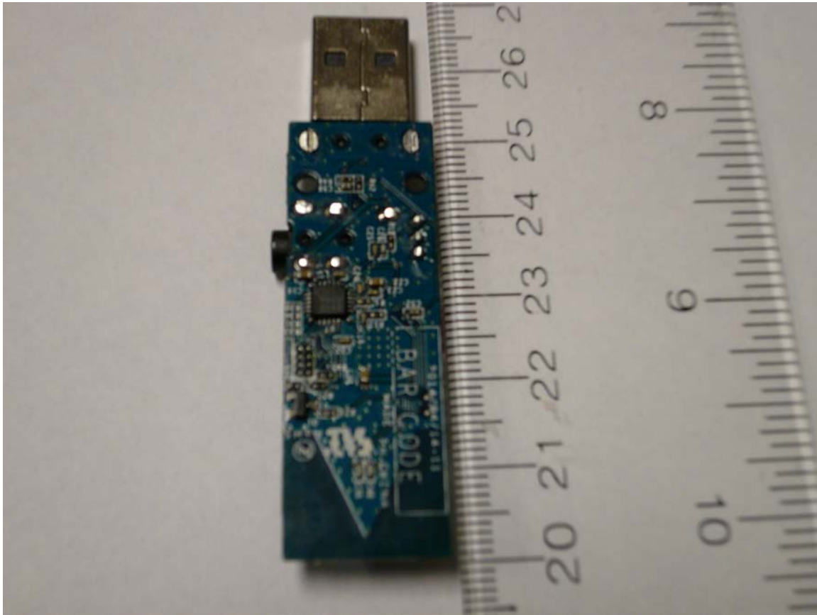
Figure 2: Internal Photo of Ear Force Stealth 500P TX - Bottom
