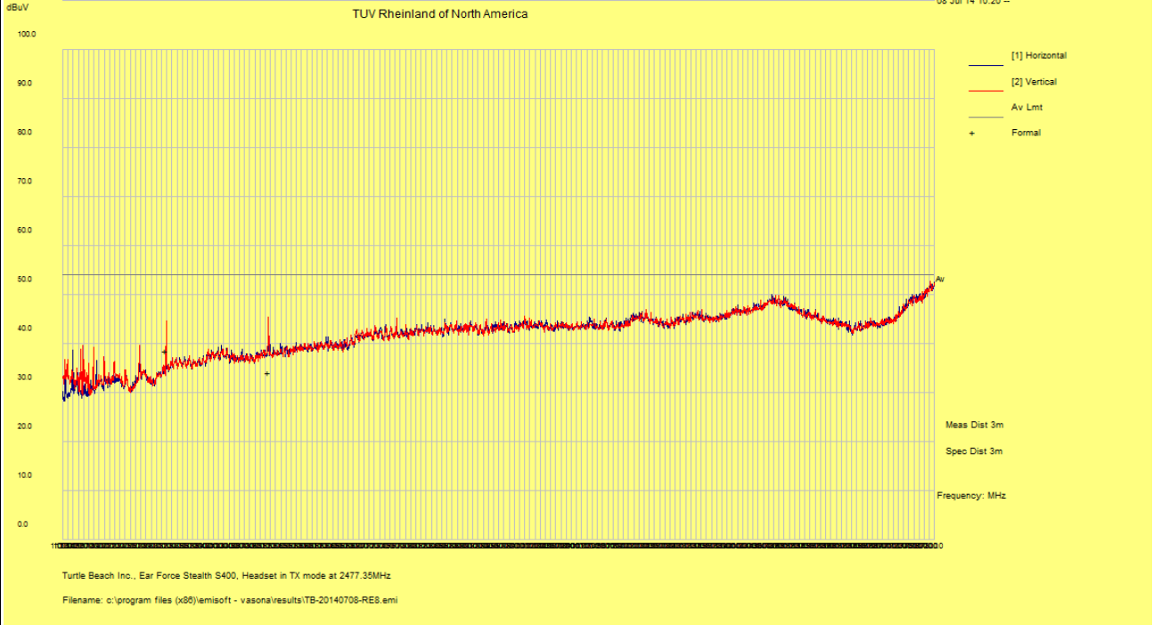
Above 1GHz Plots for Transmit Mode at 2477.35MHz
