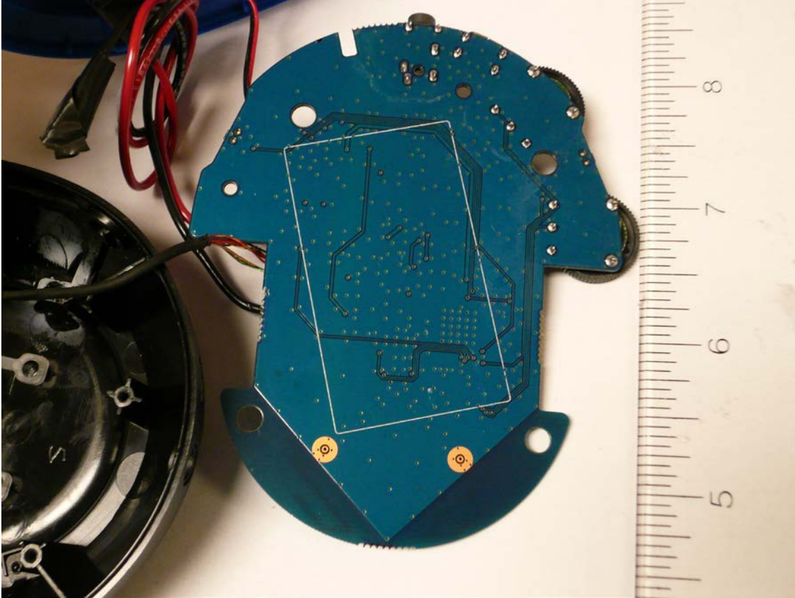
Figure 3: Internal Photo of Ear Force Stealth 500P RX without battery- Bottom
