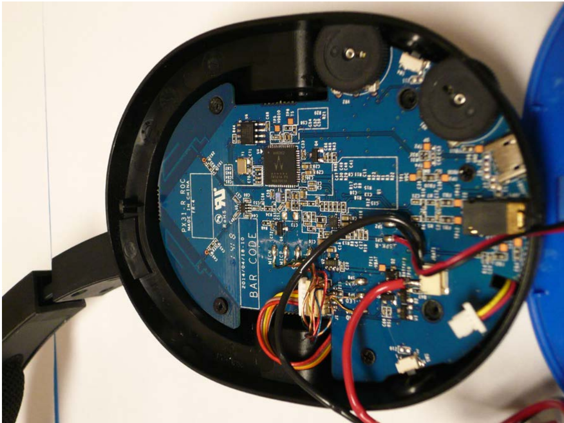
Figure 1: Internal Photo of Ear Force Stealth 500P RX - Top
