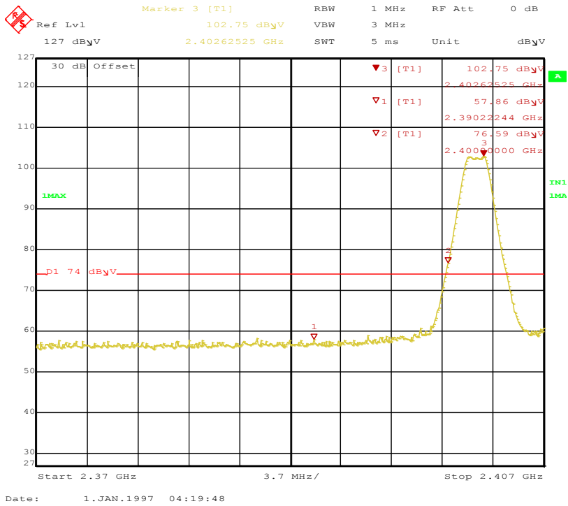
Figure 24: Band-edge-2402 MHz-H-Pk
