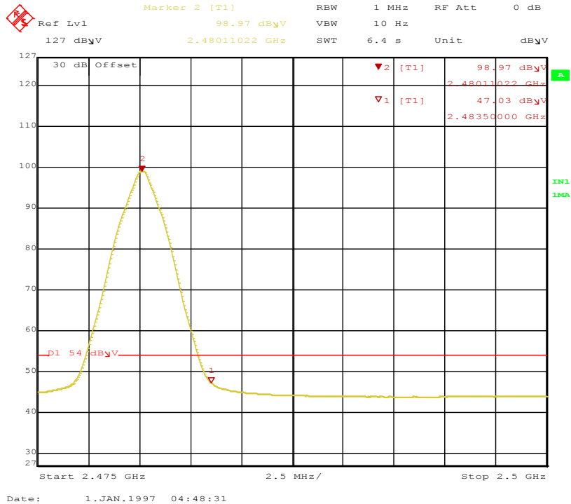
Figure 33: Band-edge-2480 MHz-H-Ave
