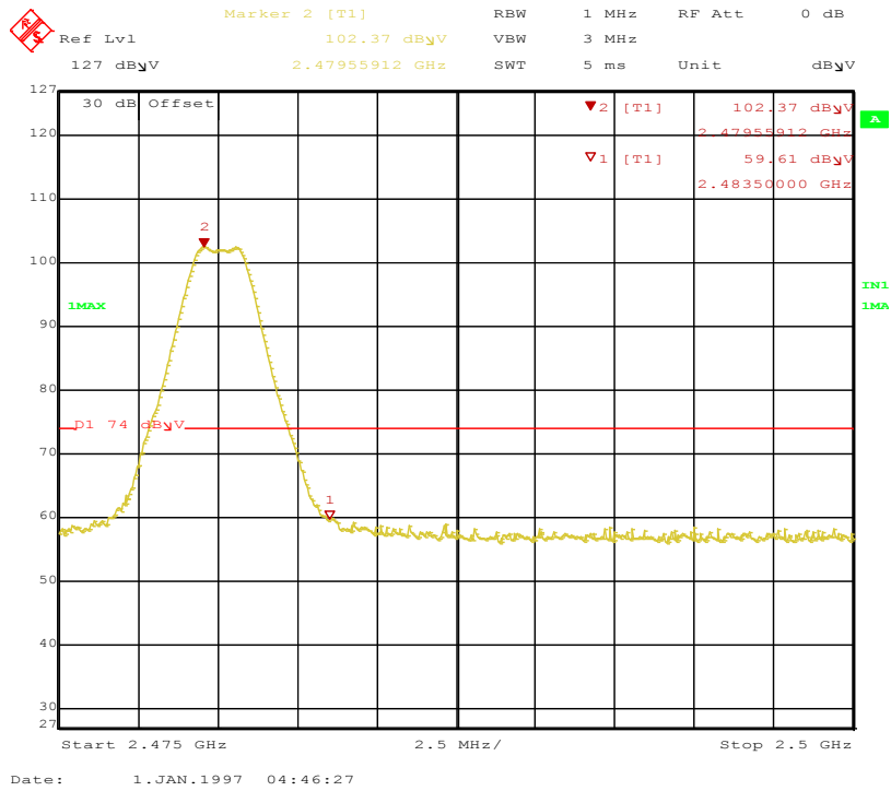
Figure 32: Band-edge-2480 MHz-H-Pk
