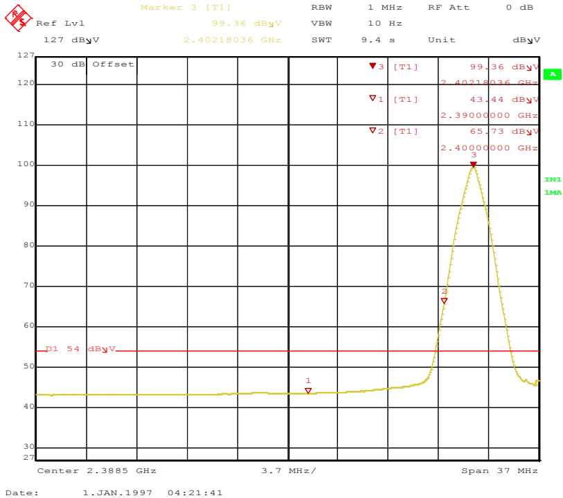
Figure 25: Band-edge-2402 MHz-H-Ave
