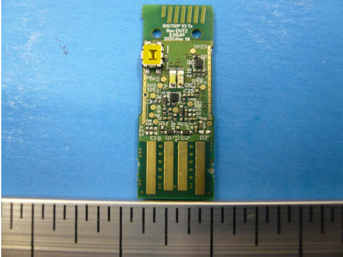
Figure 2: Internal Photo of Stealth 600P Gen 2 TX (Black & White versions) - Bottom
