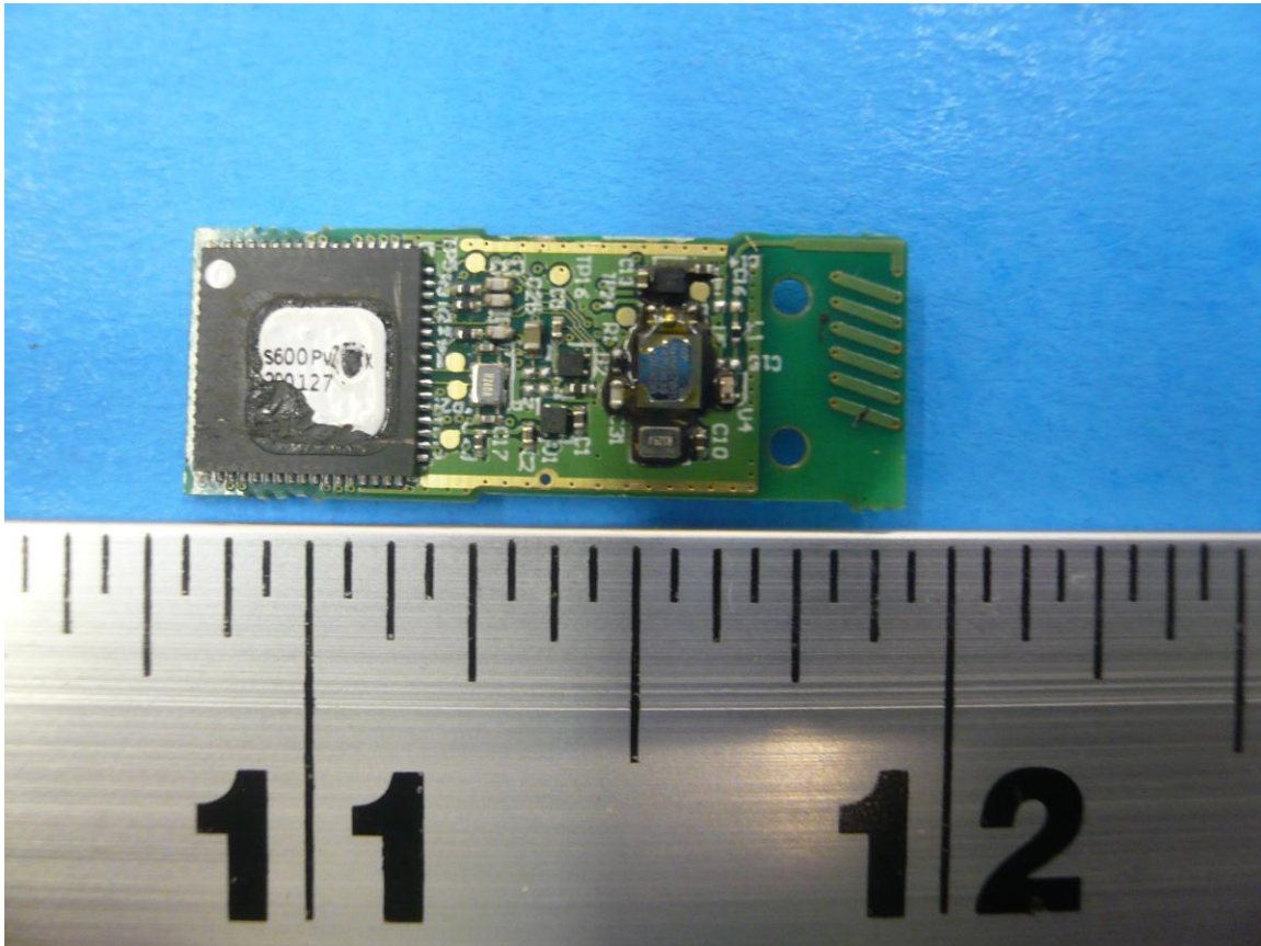
Figure 1: Internal Photo of Stealth 600P Gen 2 TX (Black & White versions) - Top
