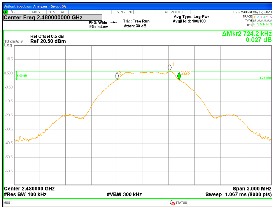
Figure 7: DTS Bandwidth-Headset -2480 MHz
