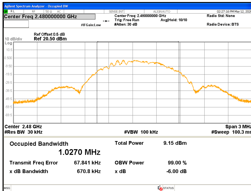
Figure 10: 99% Bandwidth-Headset -2480 MHz
