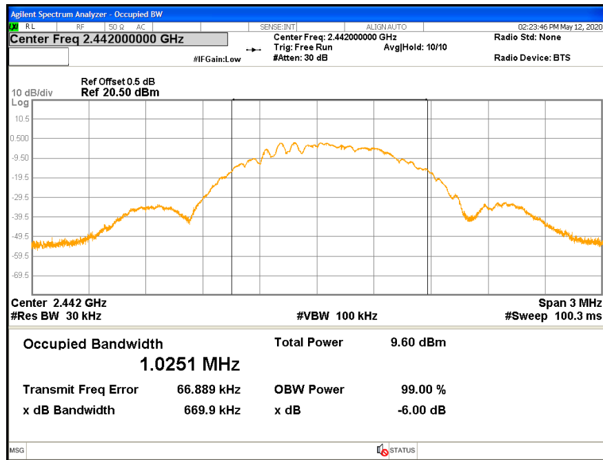
Figure 9: 99% Bandwidth-Headset -2442 MHz
