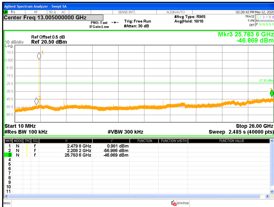
Figure 19: Out of band Emission at 2480 MHz-Headset
