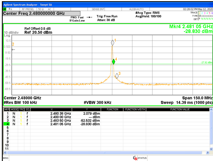
Figure 18: Conducted Band Edge at 2480 MHz-Headset
