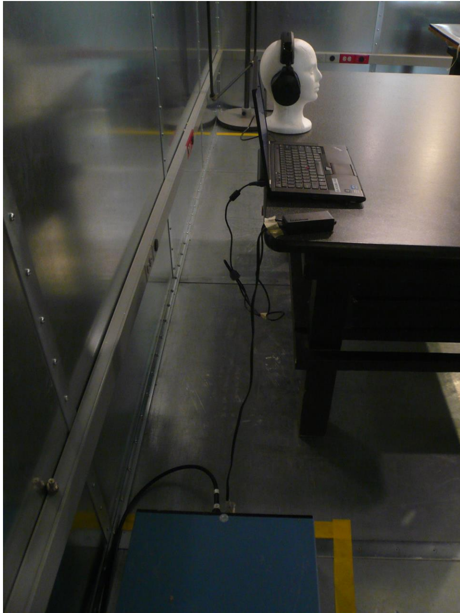
Figure 11: AC Conducted Emission Test Setup (Rear View)
