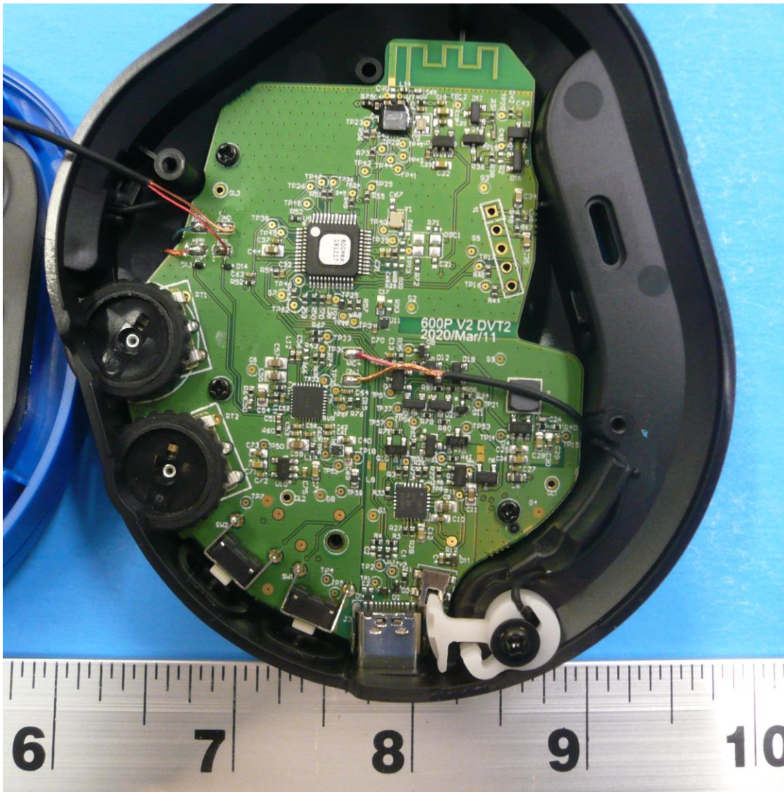
Figure 1: Internal Photo of Stealth 600P Gen 2 RX (Black & White versions) - Top
