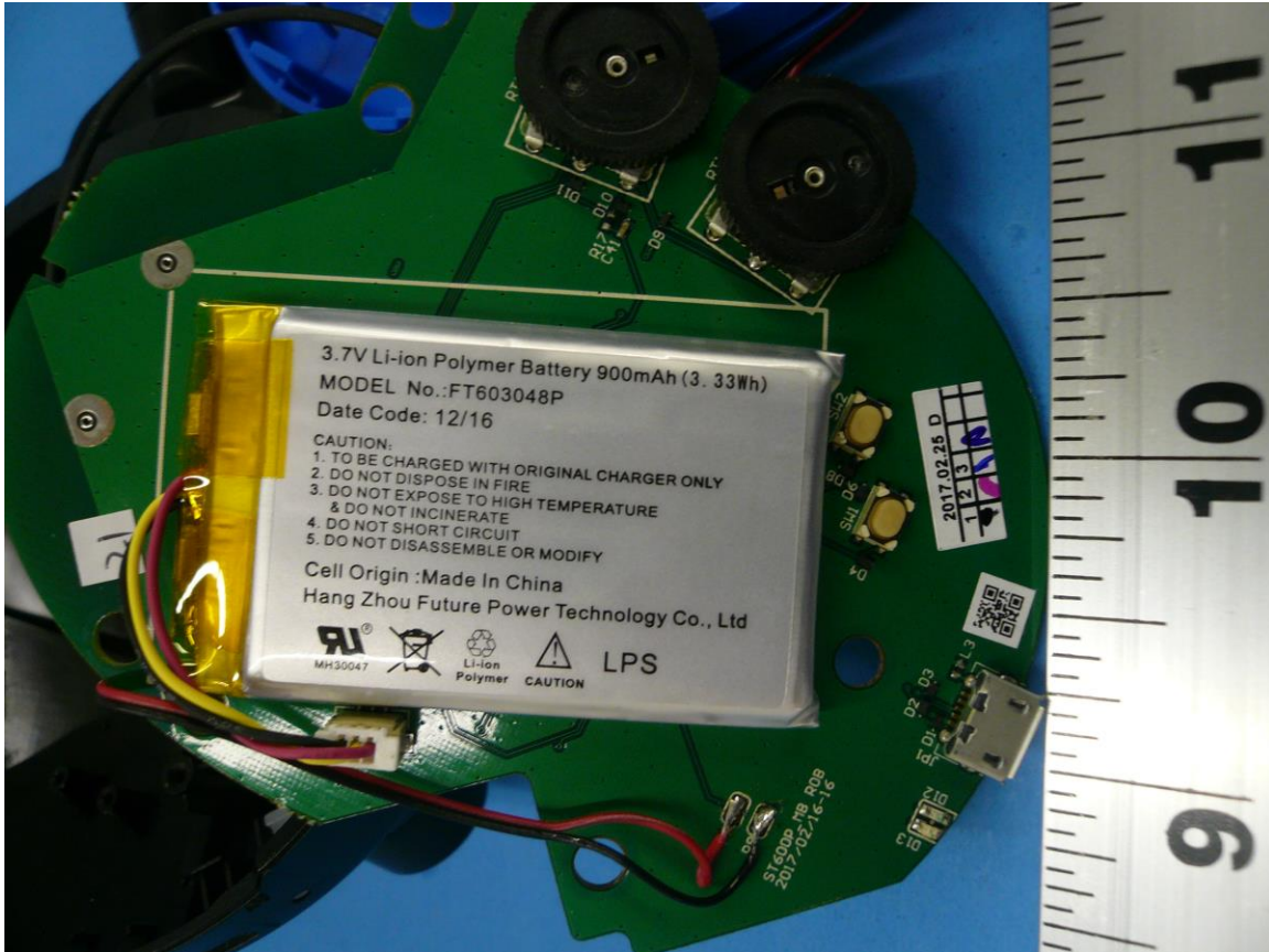
Figure 2: Internal Photo of Stealth 600P Gen 2 RX - Bottom (with battery) - (Black & White versions)
