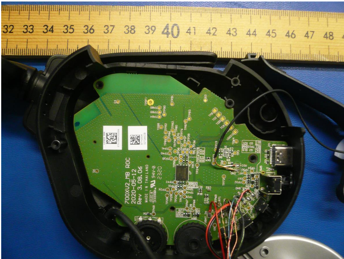
Figure 3: Internal Photo of Stealth 700X Gen 2 Main PCB (Top)
