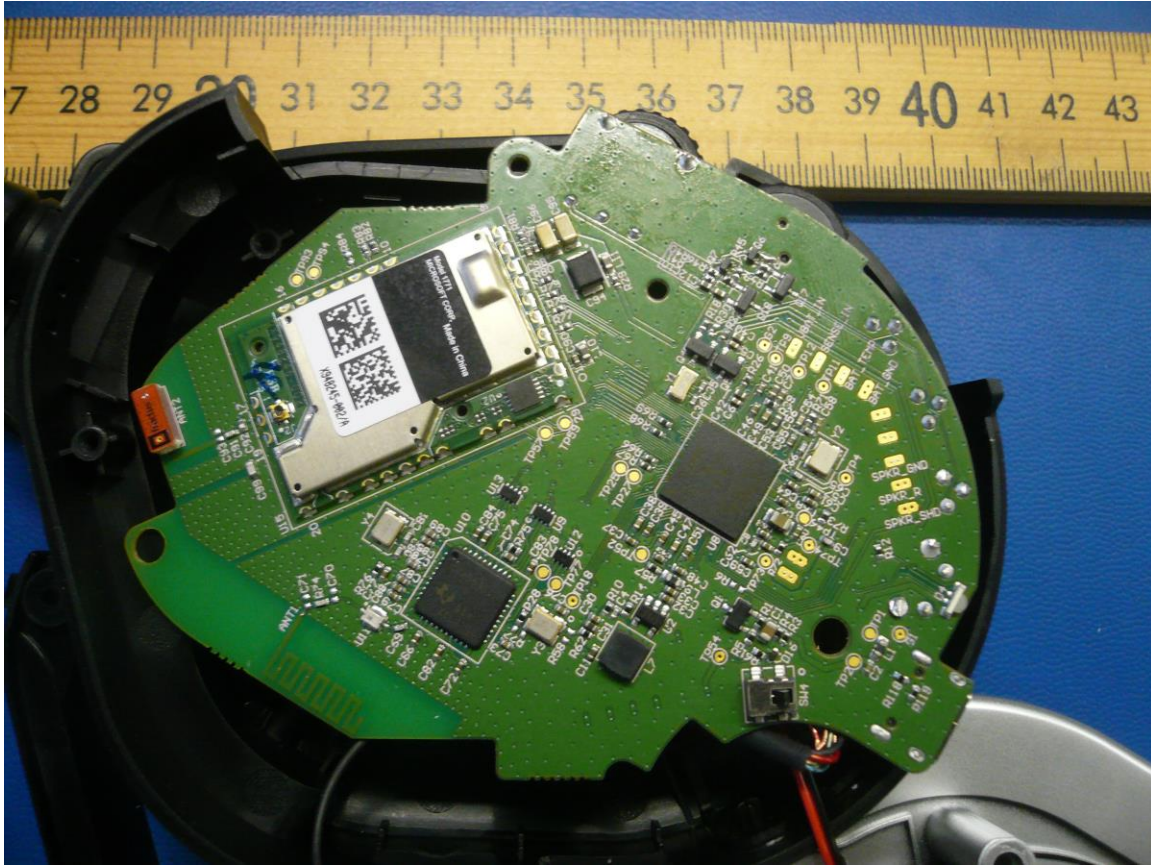
Figure 4: Internal Photo of Stealth 700X Gen 2 Main PCB (Bottom)
