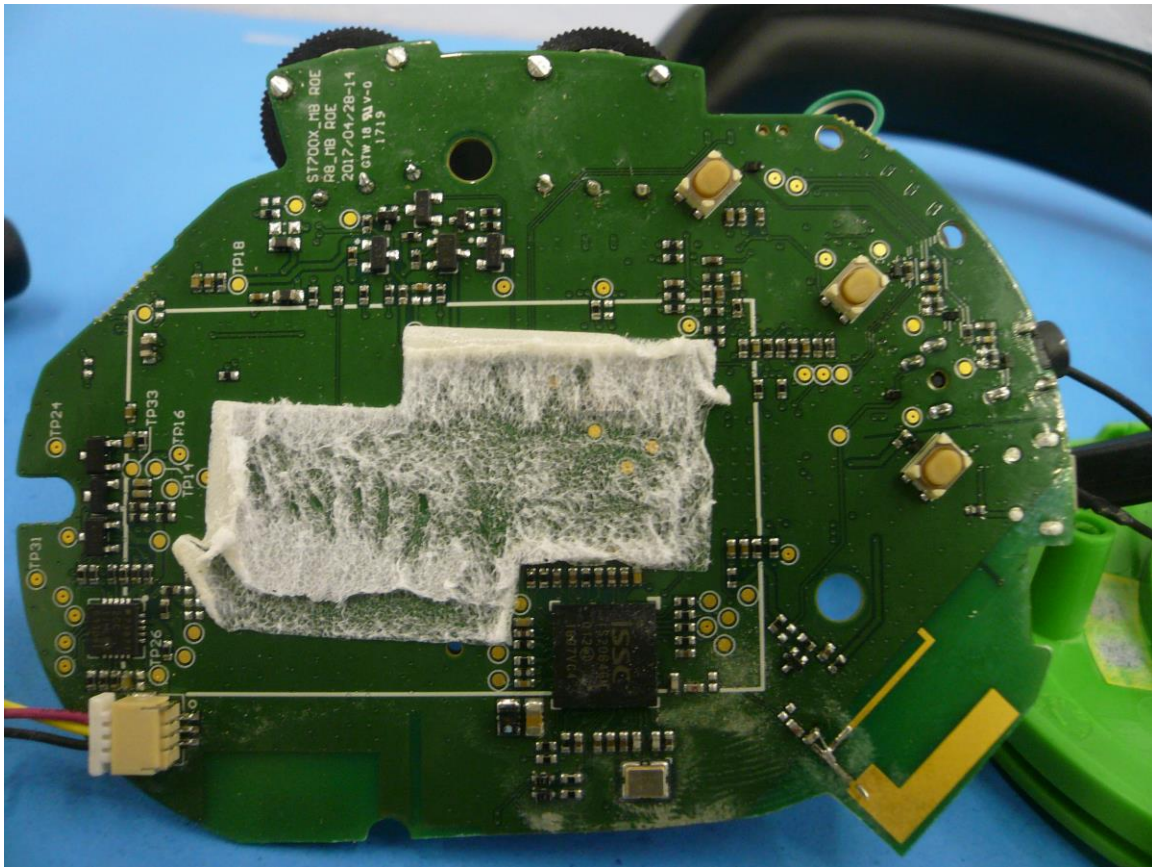
Figure 5: Internal Photo of Ear Force Stealth 700X PCB (Bottom without Battery)
