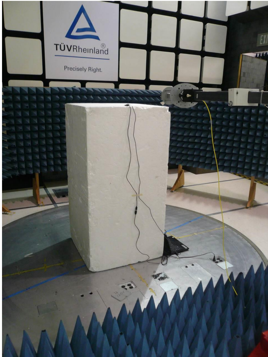
Figure 6: Test Setup for 18 GHz to 26 GHz (Rear View) - X-Axis
