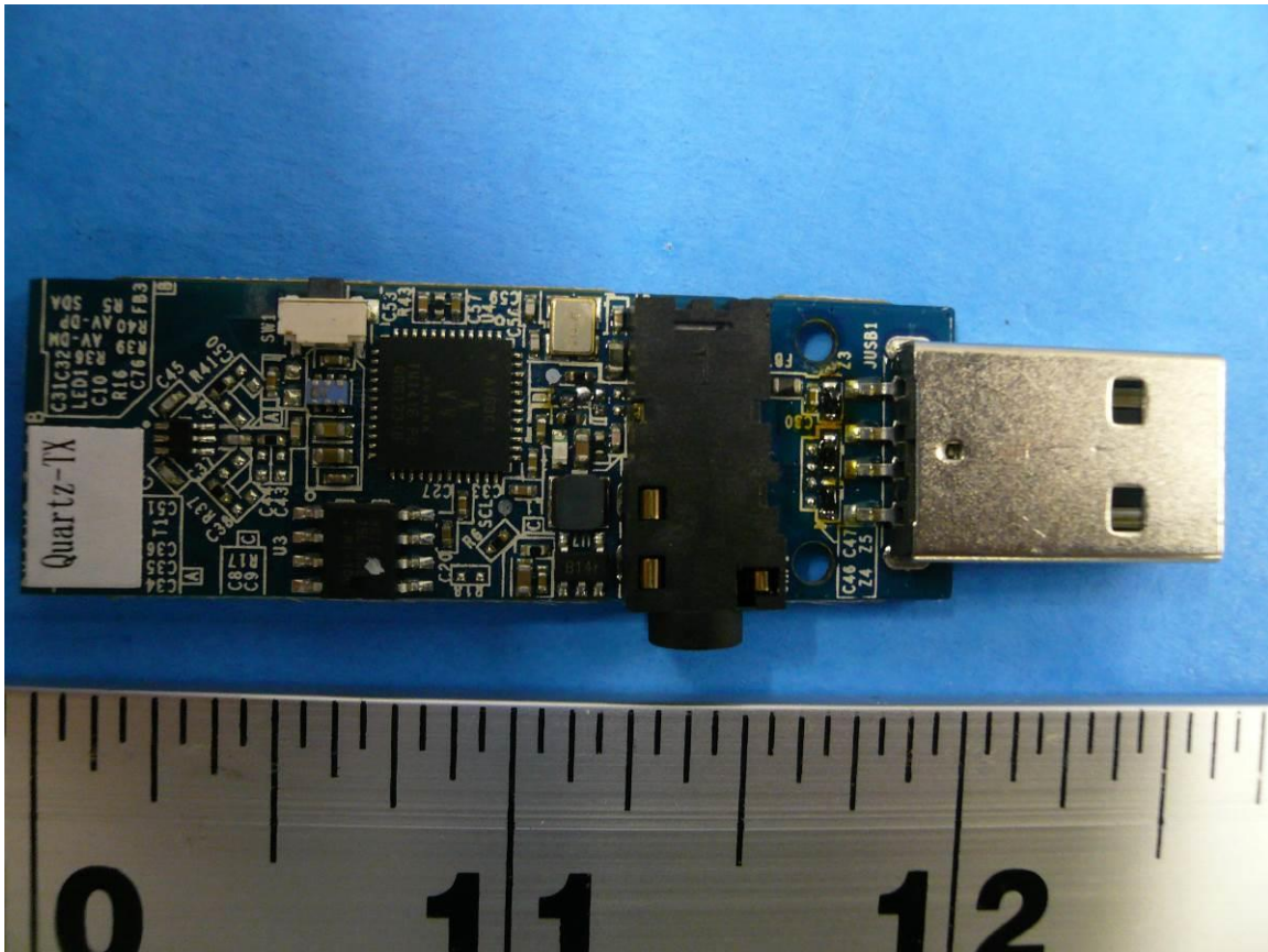
Figure 1: Internal Photo of Ear Force Stealth 520 TX - Top
