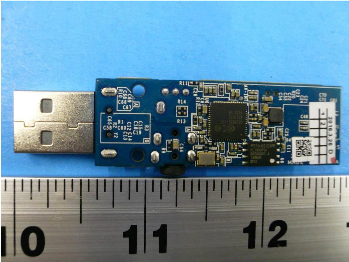
Figure 2: Internal Photo of Ear Force Stealth 520 TX - Bottom
